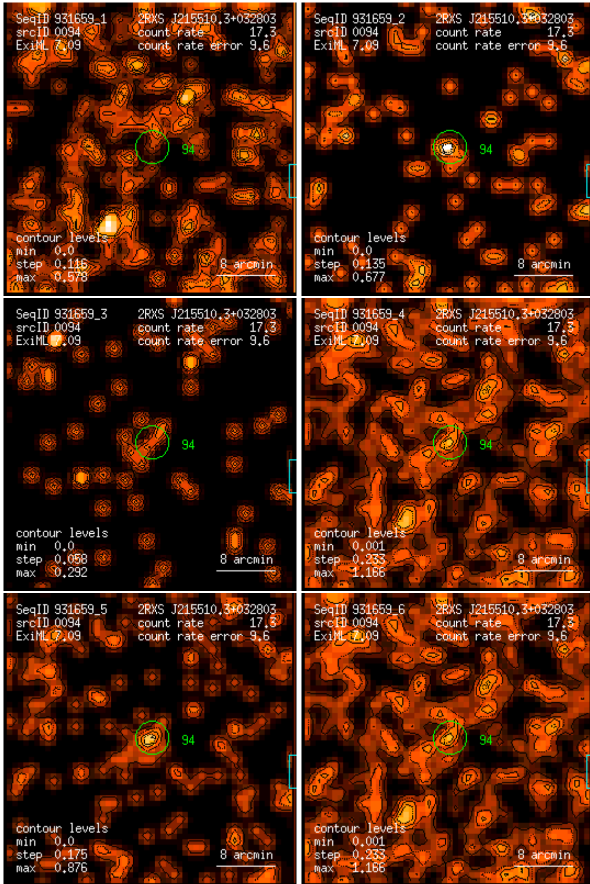
Figure 94: RASS 931659: detection 0094: band rate images, Gaussian filter: (1) PSPC channels 11 – 41, (2) 52 – 90, (3) 91 – 201, (4) 11 – 235, (5) 52 – 201, (6) 11 – 201. Broad band rates in counts/ks. Band rate contour levels in counts/ks/arcmin 2 .
