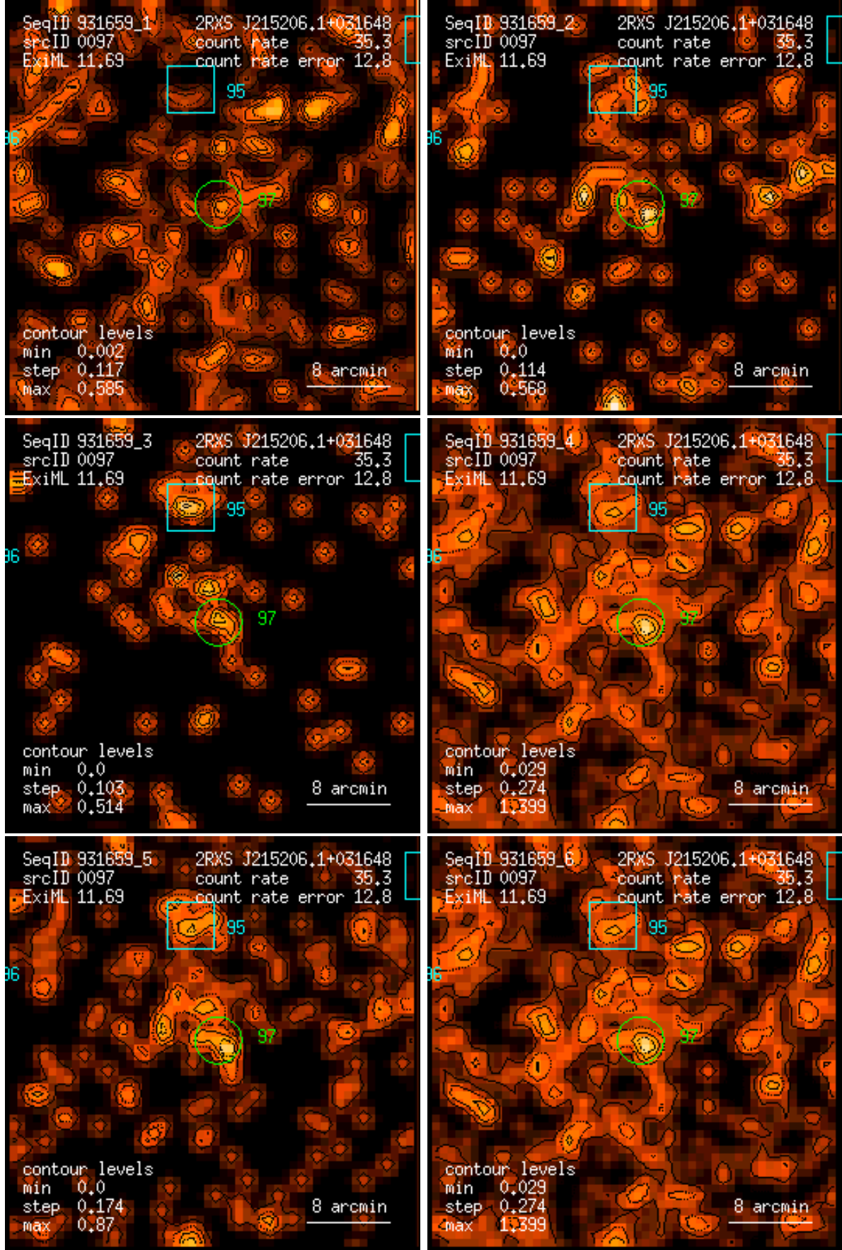
Figure 97: RASS 931659: detection 0097: band rate images, Gaussian filter: (1) PSPC channels 11 – 41, (2) 52 – 90, (3) 91 – 201, (4) 11 – 235, (5) 52 – 201, (6) 11 – 201. Broad band rates in counts/ks. Band rate contour levels in counts/ks/arcmin 2 .
