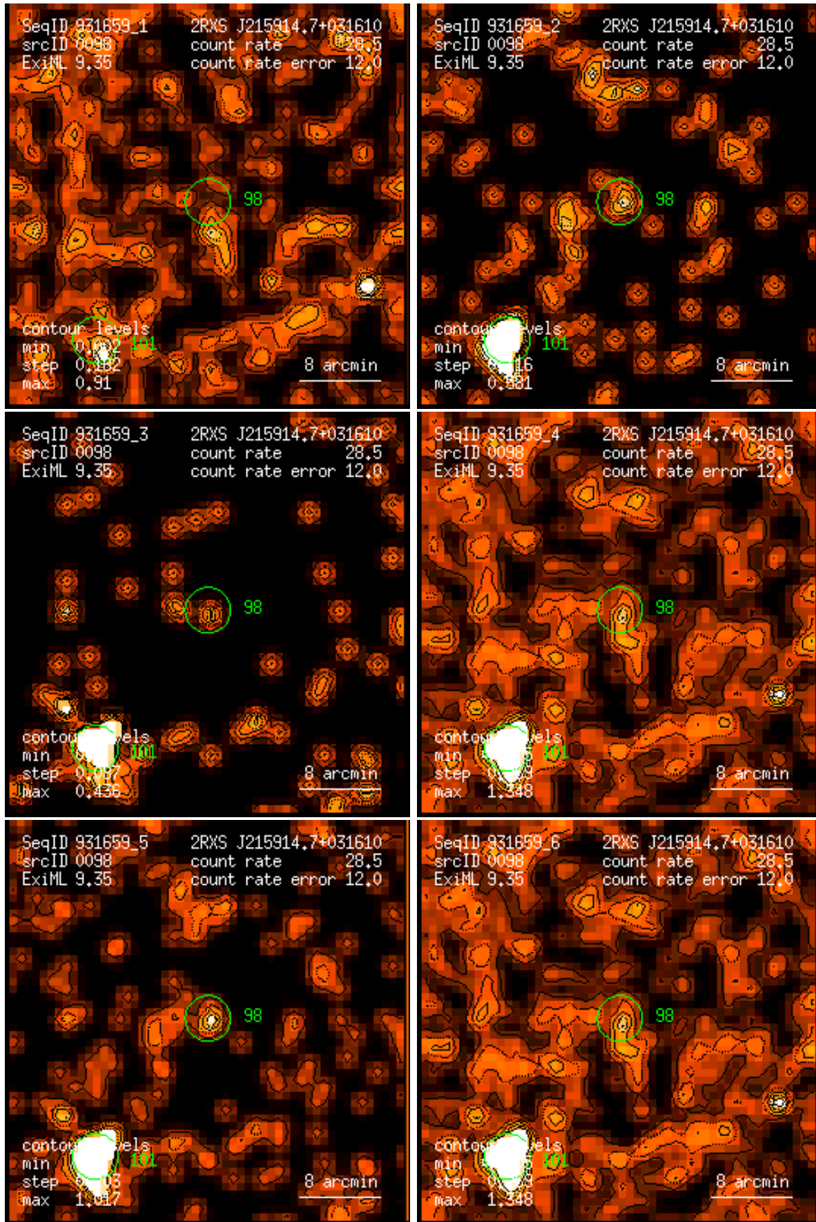
Figure 98: RASS 931659: detection 0098: band rate images, Gaussian filter: (1) PSPC channels 11 – 41, (2) 52 – 90, (3) 91 – 201, (4) 11 – 235, (5) 52 – 201, (6) 11 – 201. Broad band rates in counts/ks. Band rate contour levels in counts/ks/arcmin 2 .
