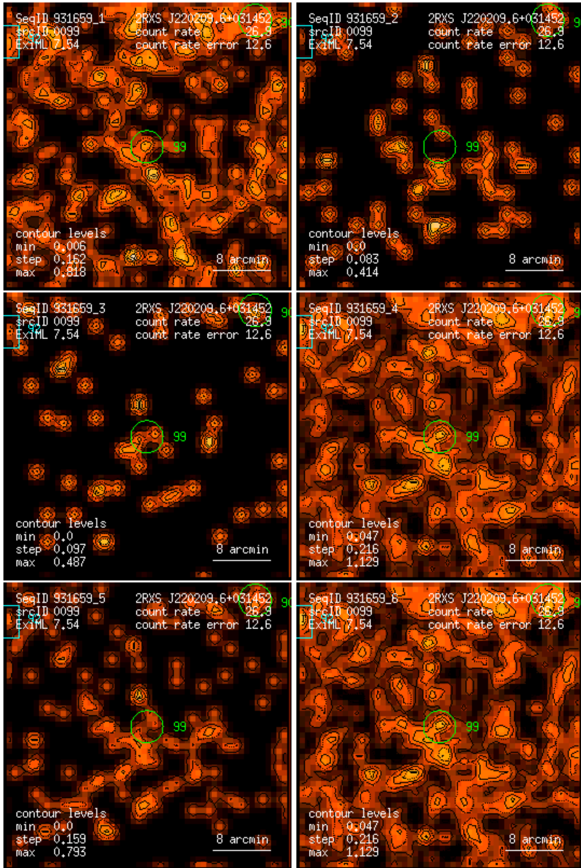
Figure 99: RASS 931659: detection 0099: band rate images, Gaussian filter: (1) PSPC channels 11 – 41, (2) 52 – 90, (3) 91 – 201, (4) 11 – 235, (5) 52 – 201, (6) 11 – 201. Broad band rates in counts/ks. Band rate contour levels in counts/ks/arcmin 2 .
