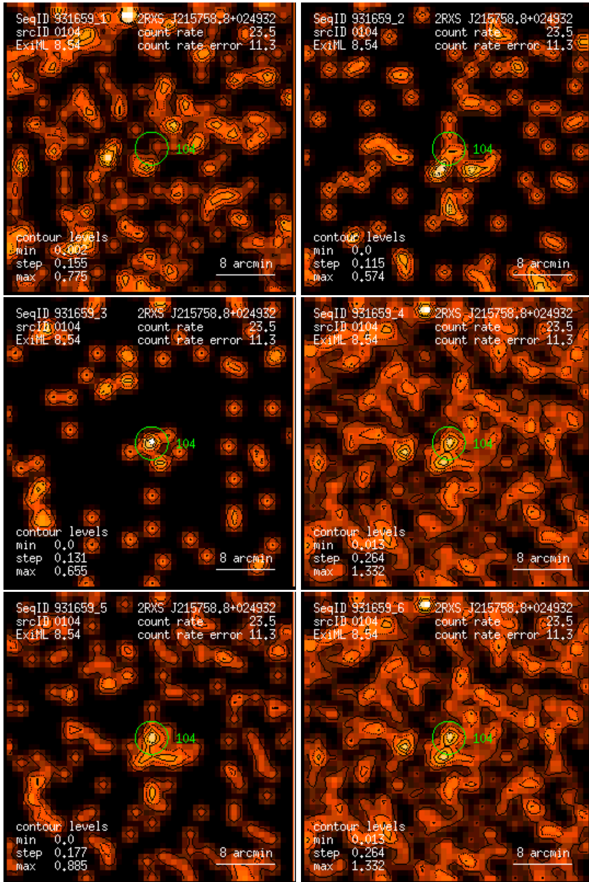
Figure 104: RASS 931659: detection 0104: band rate images, Gaussian filter: (1) PSPC channels 11 – 41, (2) 52 – 90, (3) 91 – 201, (4) 11 – 235, (5) 52 – 201, (6) 11 – 201. Broad band rates in counts/ks. Band rate contour levels in counts/ks/arcmin 2 .
