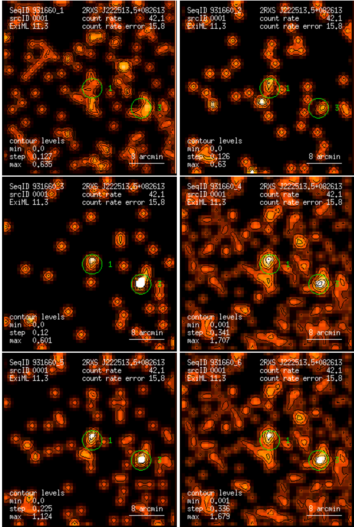
Figure 1: RASS 931660: detection 0001: band rate images, Gaussian filter: (1) PSPC channels 11 – 41, (2) 52 – 90, (3) 91 – 201, (4) 11 – 235, (5) 52 – 201, (6) 11 – 201. Broad band rates in counts/ks. Band rate contour levels in counts/ks/arcmin 2 .
