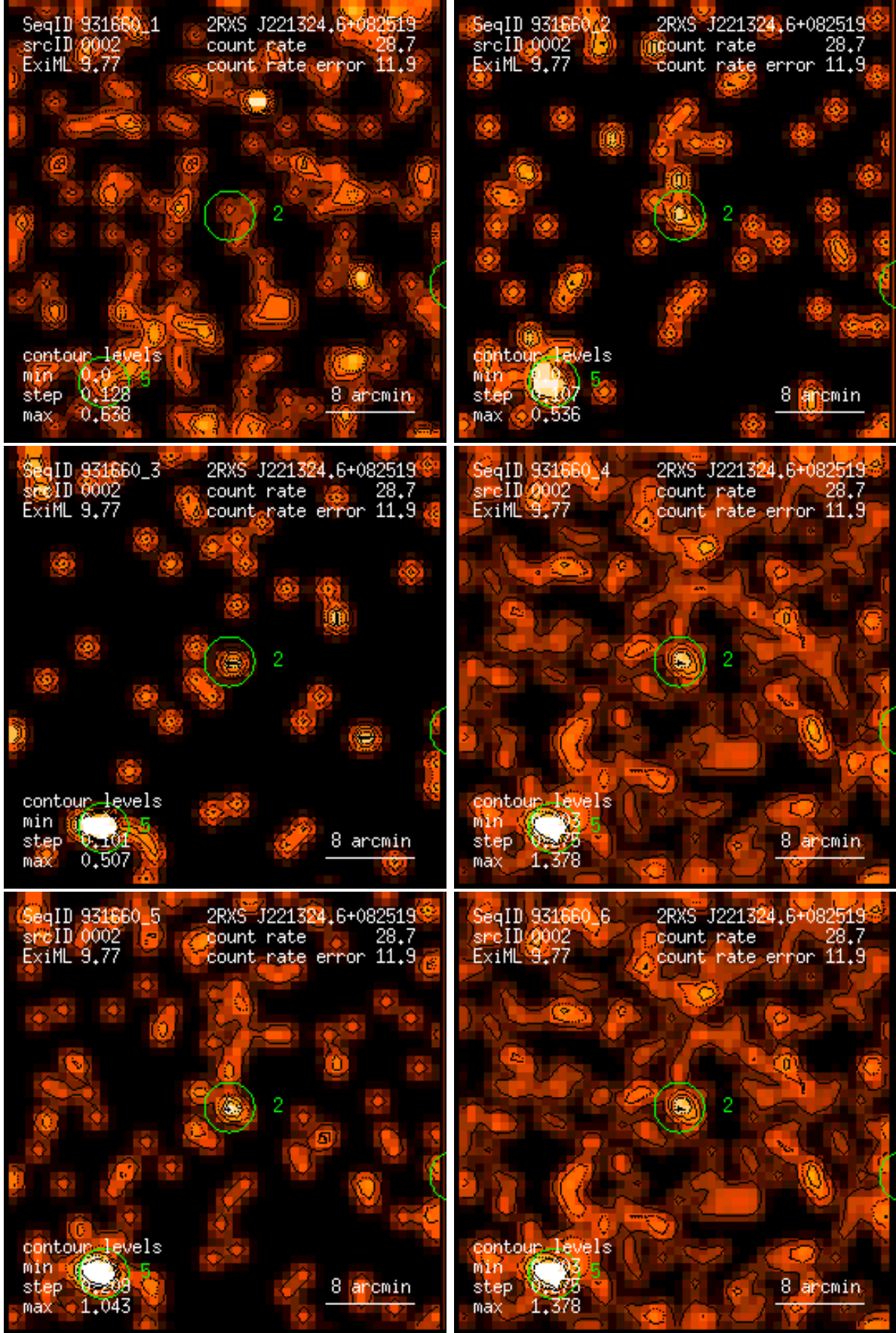
Figure 2: RASS 931660: detection 0002: band rate images, Gaussian filter: (1) PSPC channels 11 – 41, (2) 52 – 90, (3) 91 – 201, (4) 11 – 235, (5) 52 – 201, (6) 11 – 201. Broad band rates in counts/ks. Band rate contour levels in counts/ks/arcmin 2 .
