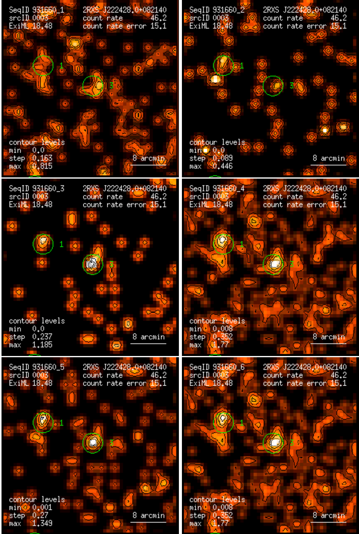
Figure 3: RASS 931660: detection 0003: band rate images, Gaussian filter: (1) PSPC channels 11 – 41, (2) 52 – 90, (3) 91 – 201, (4) 11 – 235, (5) 52 – 201, (6) 11 – 201. Broad band rates in counts/ks. Band rate contour levels in counts/ks/arcmin 2 .
