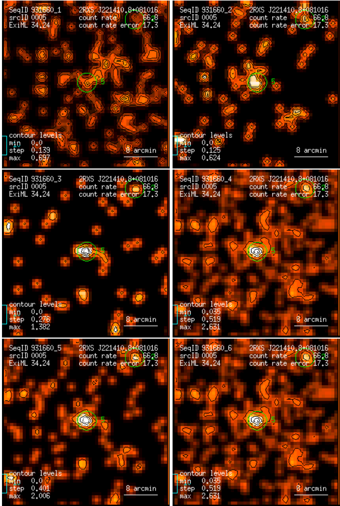
Figure 5: RASS 931660: detection 0005: band rate images, Gaussian filter: (1) PSPC channels 11 – 41, (2) 52 – 90, (3) 91 – 201, (4) 11 – 235, (5) 52 – 201, (6) 11 – 201. Broad band rates in counts/ks. Band rate contour levels in counts/ks/arcmin 2 .
