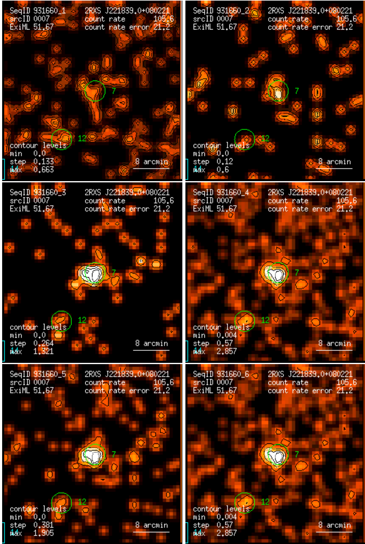
Figure 7: RASS 931660: detection 0007: band rate images, Gaussian filter: (1) PSPC channels 11 – 41, (2) 52 – 90, (3) 91 – 201, (4) 11 – 235, (5) 52 – 201, (6) 11 – 201. Broad band rates in counts/ks. Band rate contour levels in counts/ks/arcmin 2 .
