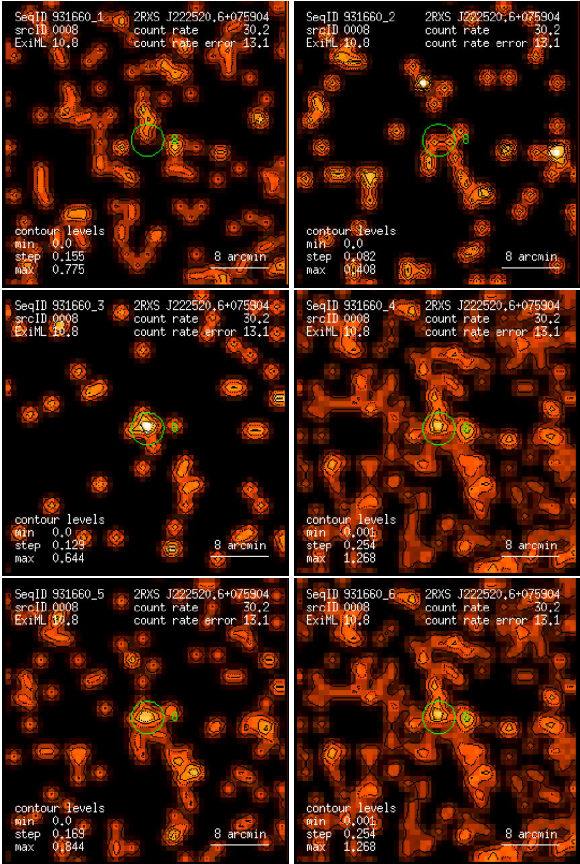
Figure 8: RASS 931660: detection 0008: band rate images, Gaussian filter: (1) PSPC channels 11 – 41, (2) 52 – 90, (3) 91 – 201, (4) 11 – 235, (5) 52 – 201, (6) 11 – 201. Broad band rates in counts/ks. Band rate contour levels in counts/ks/arcmin 2 .
