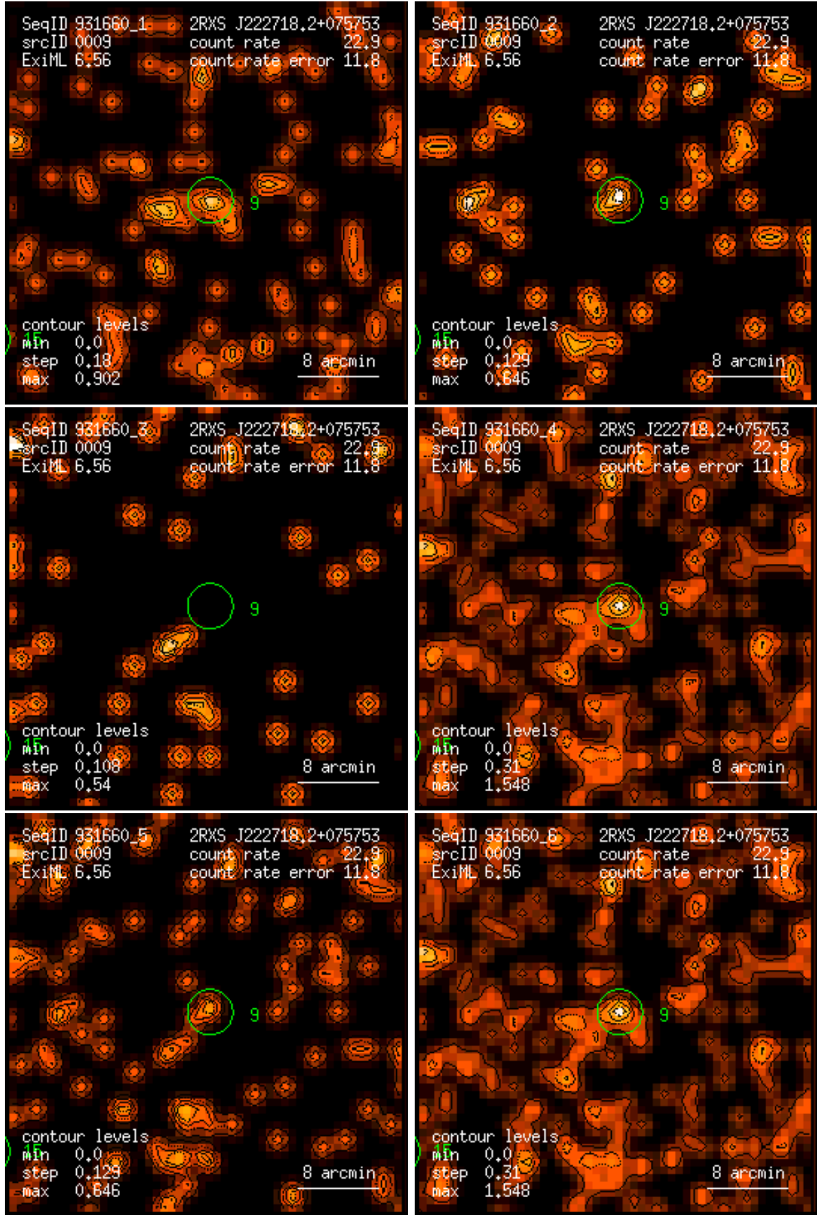
Figure 9: RASS 931660: detection 0009: band rate images, Gaussian filter: (1) PSPC channels 11 – 41, (2) 52 – 90, (3) 91 – 201, (4) 11 – 235, (5) 52 – 201, (6) 11 – 201. Broad band rates in counts/ks. Band rate contour levels in counts/ks/arcmin 2 .
