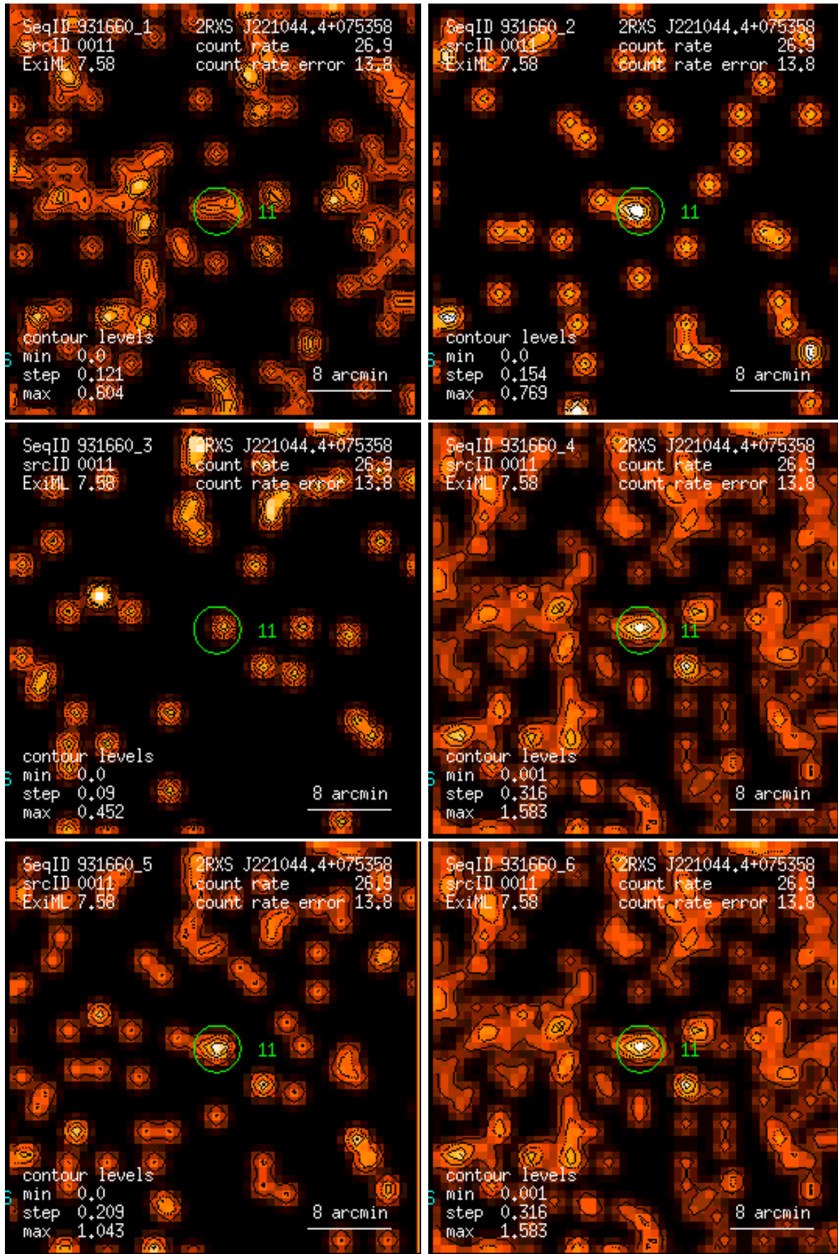
Figure 11: RASS 931660: detection 0011: band rate images, Gaussian filter: (1) PSPC channels 11 – 41, (2) 52 – 90, (3) 91 – 201, (4) 11 – 235, (5) 52 – 201, (6) 11 – 201. Broad band rates in counts/ks. Band rate contour levels in counts/ks/arcmin 2 .
