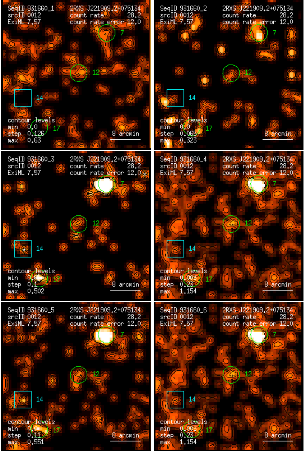
Figure 12: RASS 931660: detection 0012: band rate images, Gaussian filter: (1) PSPC channels 11 – 41, (2) 52 – 90, (3) 91 – 201, (4) 11 – 235, (5) 52 – 201, (6) 11 – 201. Broad band rates in counts/ks. Band rate contour levels in counts/ks/arcmin 2 .
