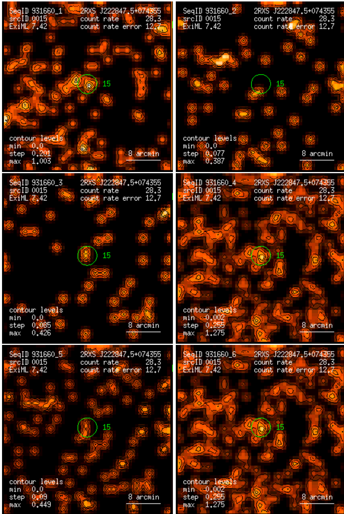
Figure 15: RASS 931660: detection 0015: band rate images, Gaussian filter: (1) PSPC channels 11 – 41, (2) 52 – 90, (3) 91 – 201, (4) 11 – 235, (5) 52 – 201, (6) 11 – 201. Broad band rates in counts/ks. Band rate contour levels in counts/ks/arcmin 2 .
