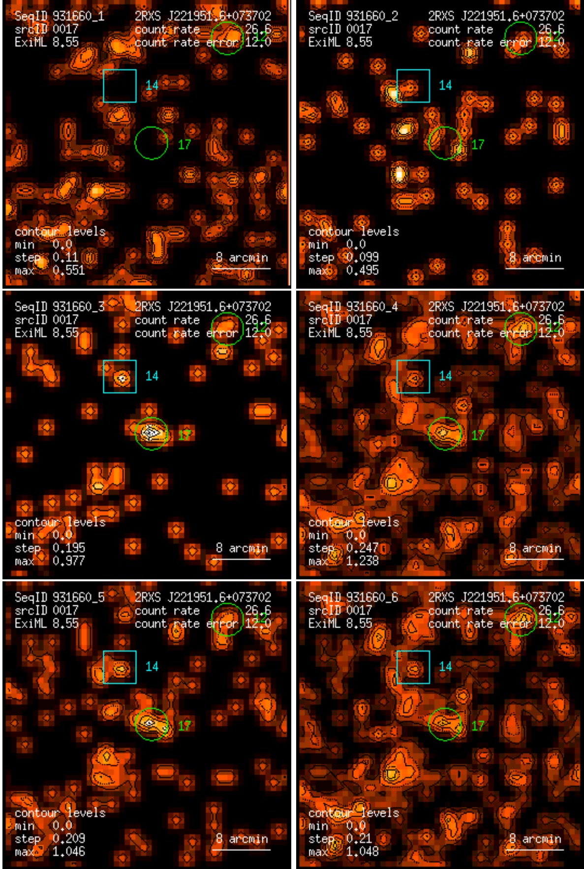
Figure 17: RASS 931660: detection 0017: band rate images, Gaussian filter: (1) PSPC channels 11 – 41, (2) 52 – 90, (3) 91 – 201, (4) 11 – 235, (5) 52 – 201, (6) 11 – 201. Broad band rates in counts/ks. Band rate contour levels in counts/ks/arcmin 2 .
