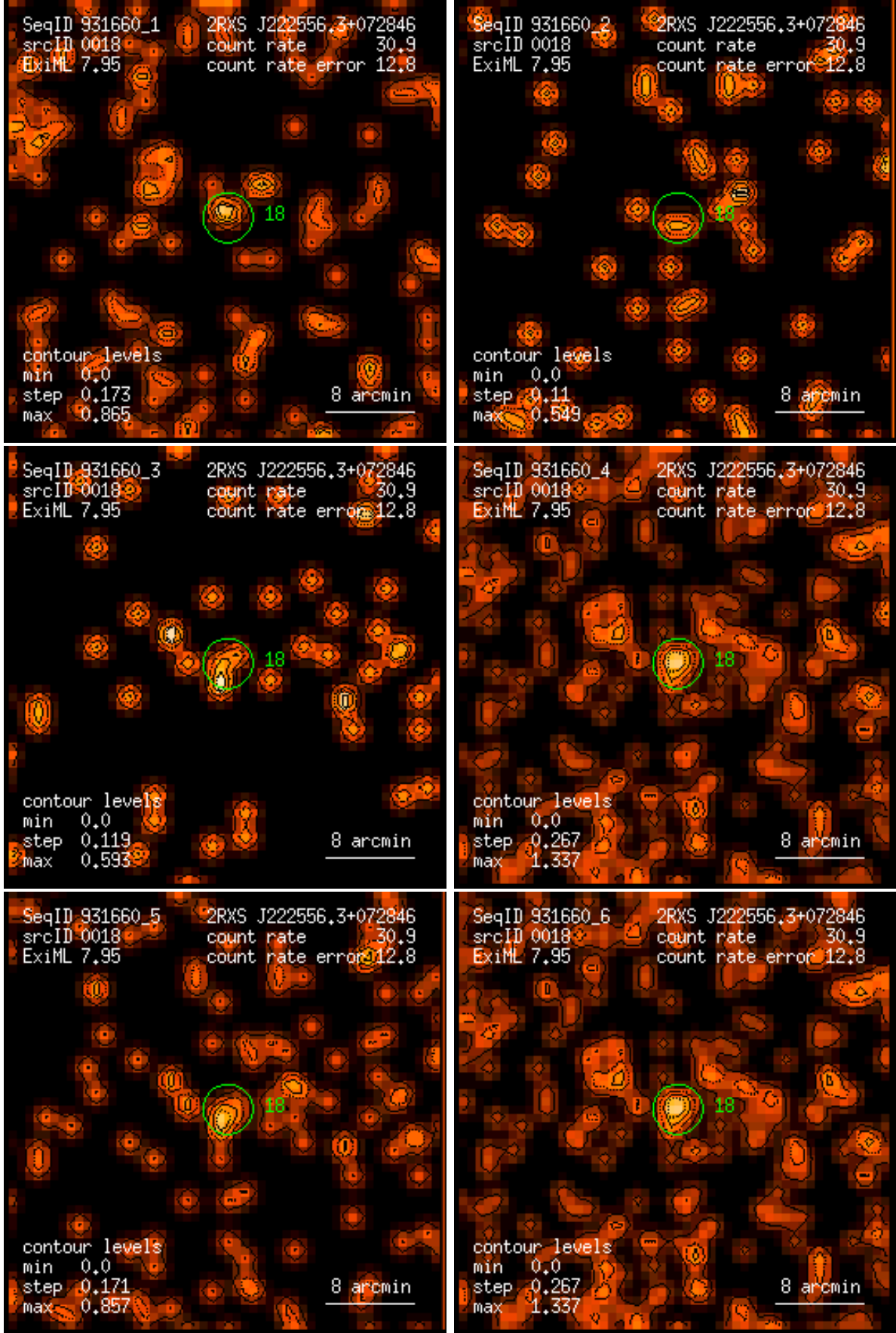
Figure 18: RASS 931660: detection 0018: band rate images, Gaussian filter: (1) PSPC channels 11 – 41, (2) 52 – 90, (3) 91 – 201, (4) 11 – 235, (5) 52 – 201, (6) 11 – 201. Broad band rates in counts/ks. Band rate contour levels in counts/ks/arcmin 2 .
