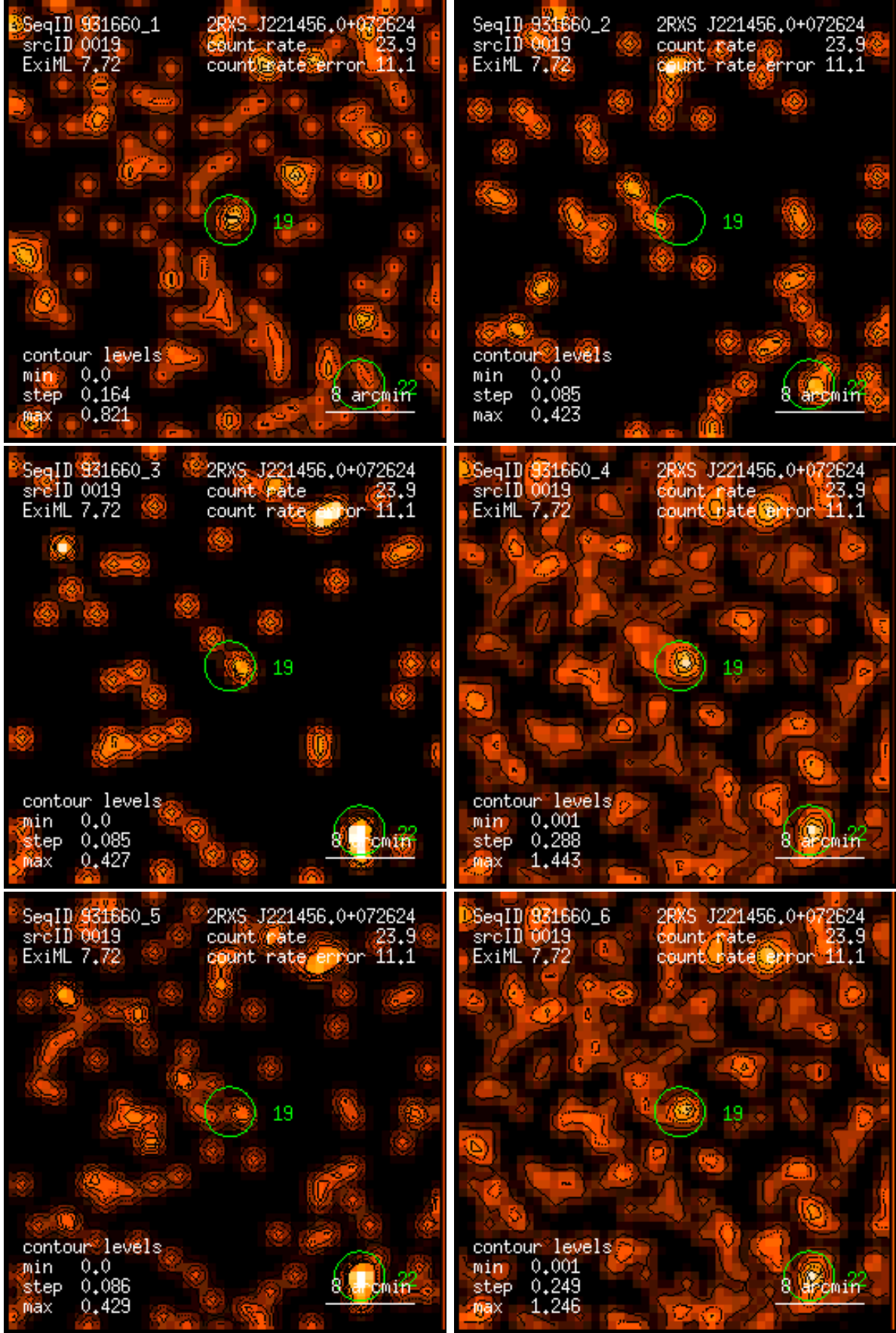
Figure 19: RASS 931660: detection 0019: band rate images, Gaussian filter: (1) PSPC channels 11 – 41, (2) 52 – 90, (3) 91 – 201, (4) 11 – 235, (5) 52 – 201, (6) 11 – 201. Broad band rates in counts/ks. Band rate contour levels in counts/ks/arcmin 2 .
