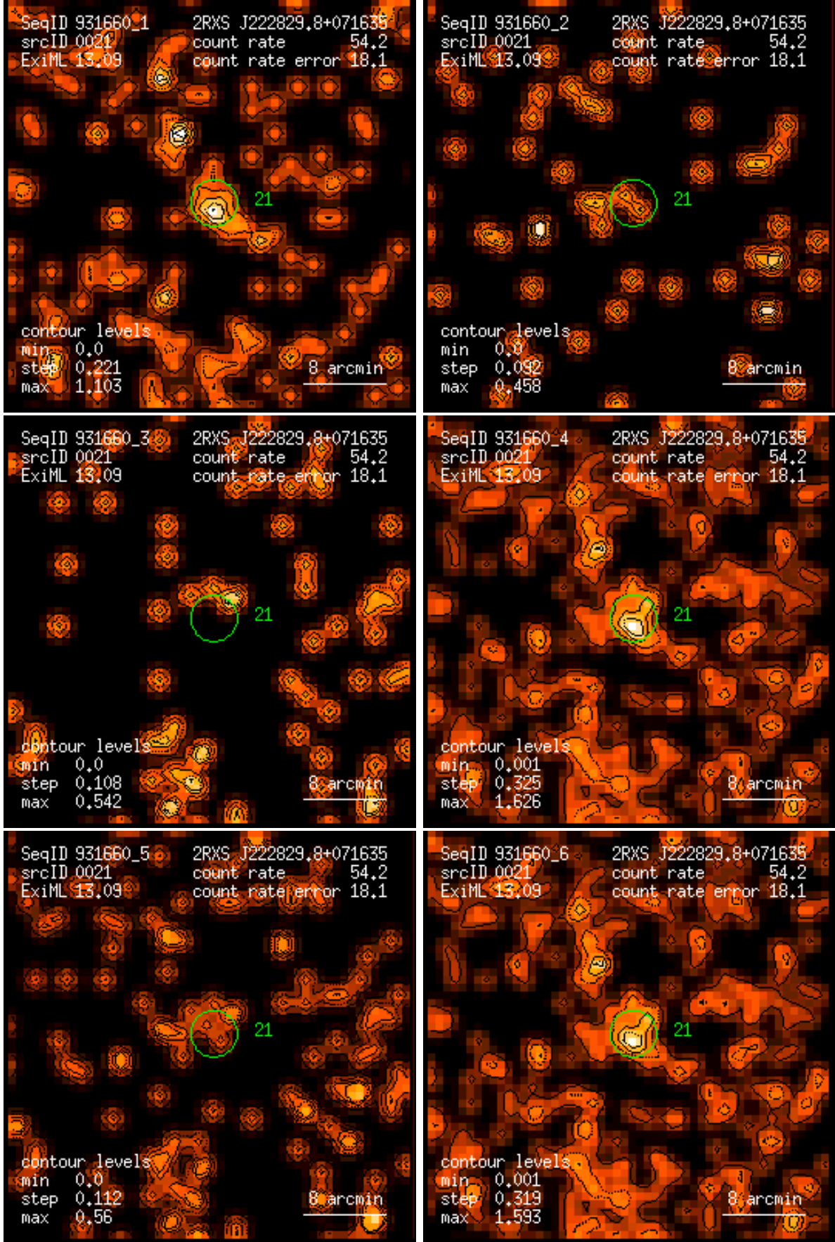
Figure 21: RASS 931660: detection 0021: band rate images, Gaussian filter: (1) PSPC channels 11 – 41, (2) 52 – 90, (3) 91 – 201, (4) 11 – 235, (5) 52 – 201, (6) 11 – 201. Broad band rates in counts/ks. Band rate contour levels in counts/ks/arcmin 2 .
