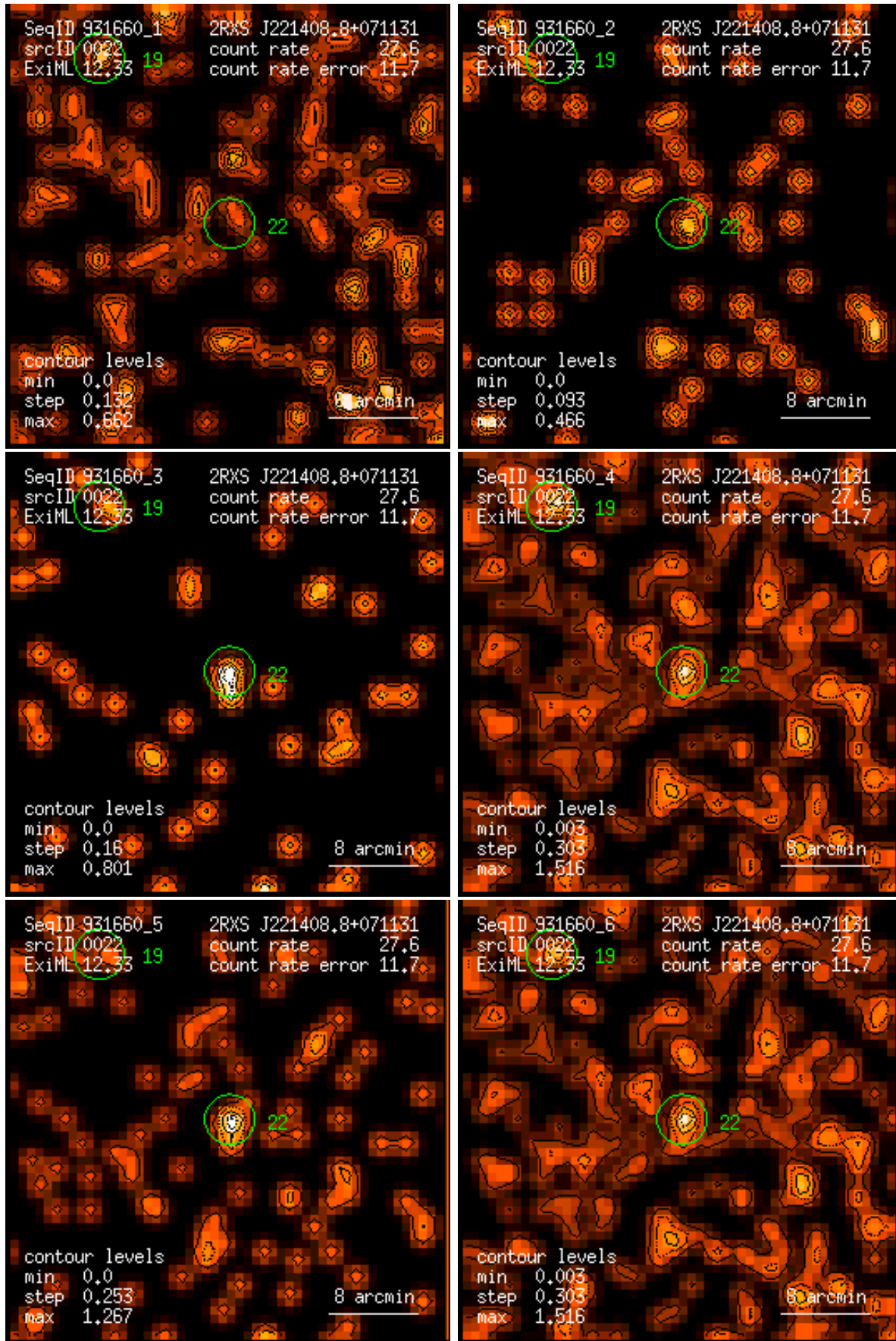
Figure 22: RASS 931660: detection 0022: band rate images, Gaussian filter: (1) PSPC channels 11 – 41, (2) 52 – 90, (3) 91 – 201, (4) 11 – 235, (5) 52 – 201, (6) 11 – 201. Broad band rates in counts/ks. Band rate contour levels in counts/ks/arcmin 2 .
