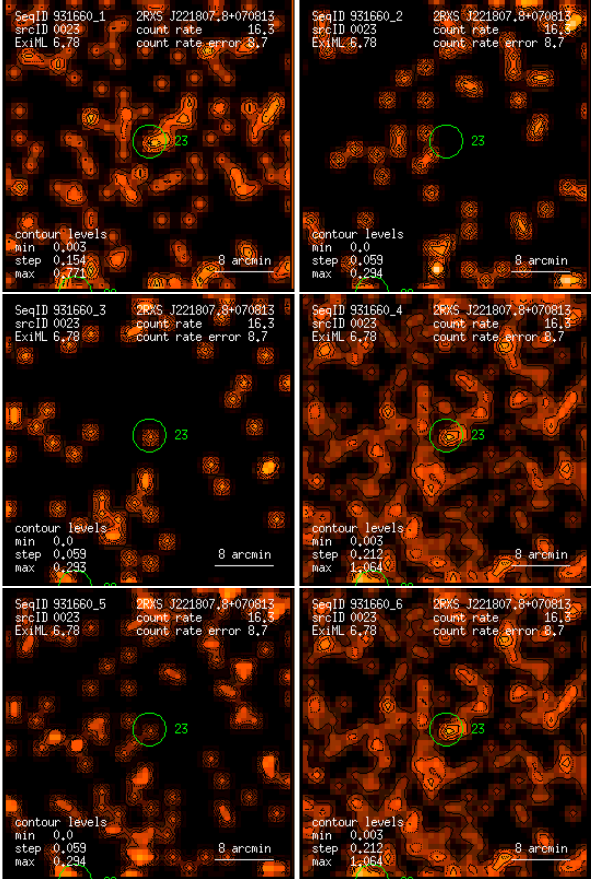
Figure 23: RASS 931660: detection 0023: band rate images, Gaussian filter: (1) PSPC channels 11 – 41, (2) 52 – 90, (3) 91 – 201, (4) 11 – 235, (5) 52 – 201, (6) 11 – 201. Broad band rates in counts/ks. Band rate contour levels in counts/ks/arcmin 2 .
