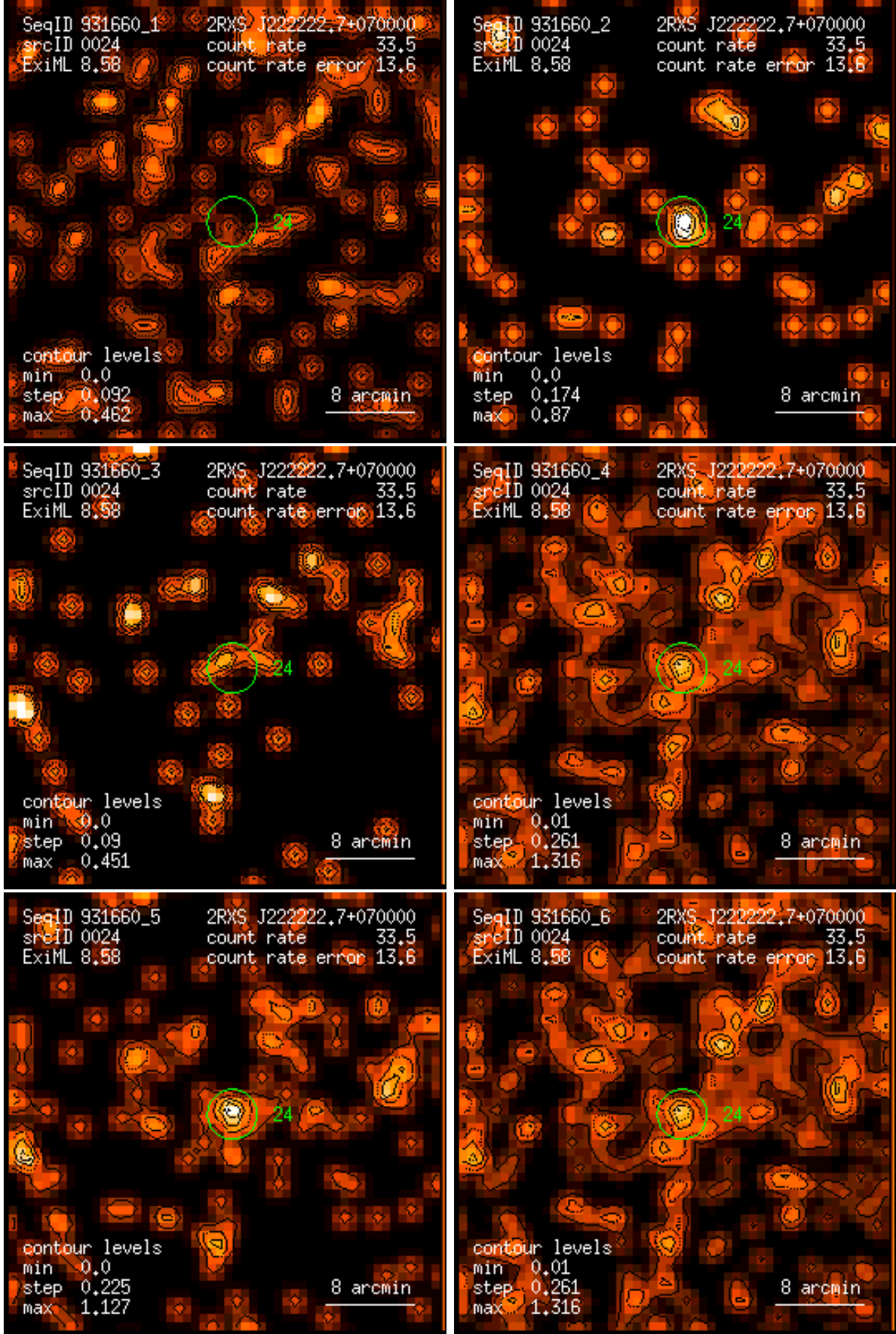
Figure 24: RASS 931660: detection 0024: band rate images, Gaussian filter: (1) PSPC channels 11 – 41, (2) 52 – 90, (3) 91 – 201, (4) 11 – 235, (5) 52 – 201, (6) 11 – 201. Broad band rates in counts/ks. Band rate contour levels in counts/ks/arcmin 2 .
