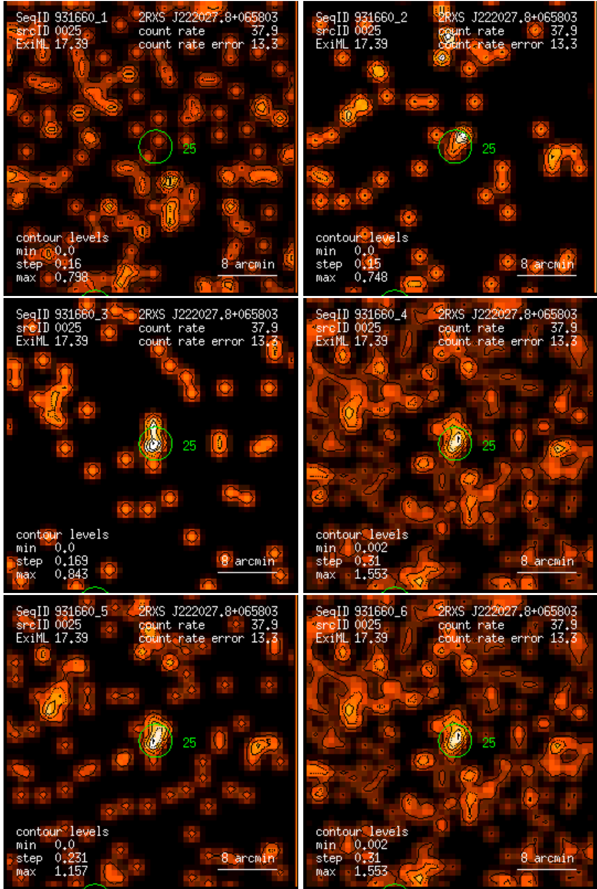
Figure 25: RASS 931660: detection 0025: band rate images, Gaussian filter: (1) PSPC channels 11 – 41, (2) 52 – 90, (3) 91 – 201, (4) 11 – 235, (5) 52 – 201, (6) 11 – 201. Broad band rates in counts/ks. Band rate contour levels in counts/ks/arcmin 2 .
