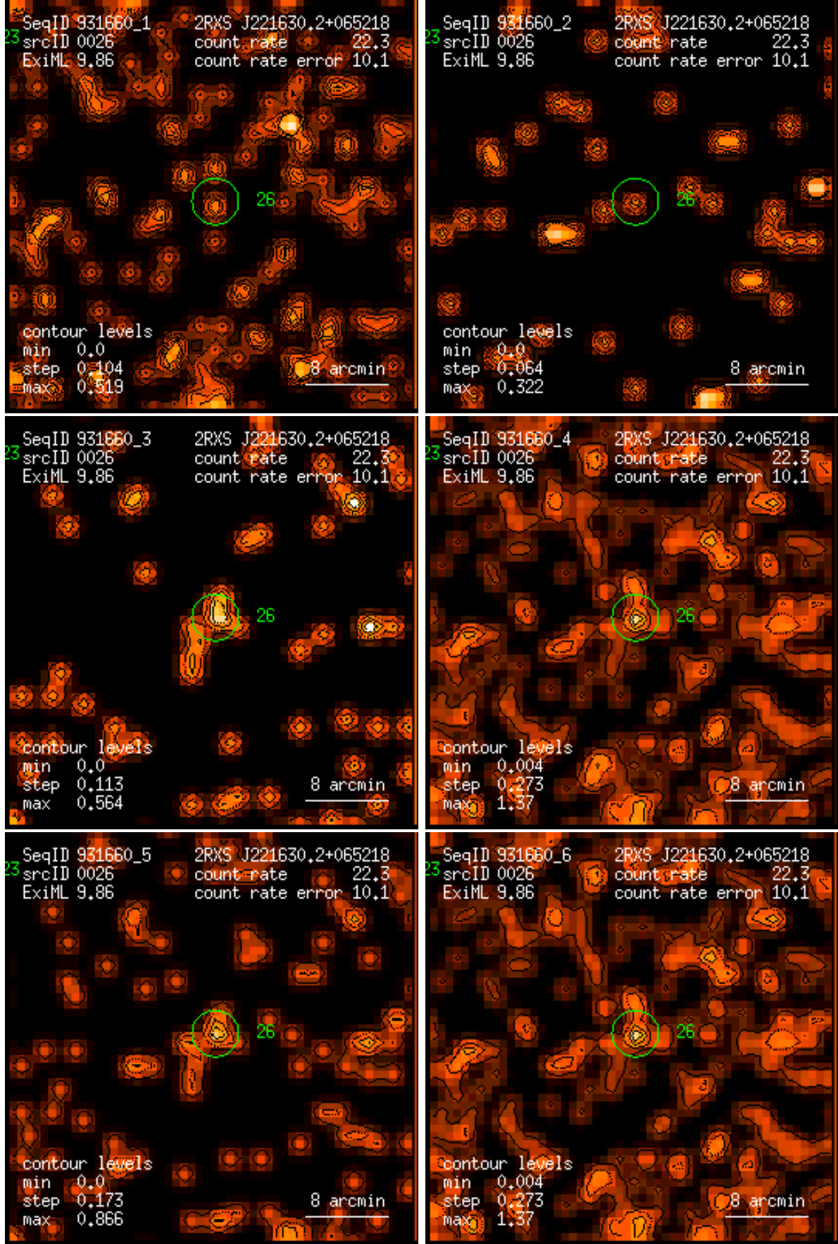
Figure 26: RASS 931660: detection 0026: band rate images, Gaussian filter: (1) PSPC channels 11 – 41, (2) 52 – 90, (3) 91 – 201, (4) 11 – 235, (5) 52 – 201, (6) 11 – 201. Broad band rates in counts/ks. Band rate contour levels in counts/ks/arcmin 2 .
