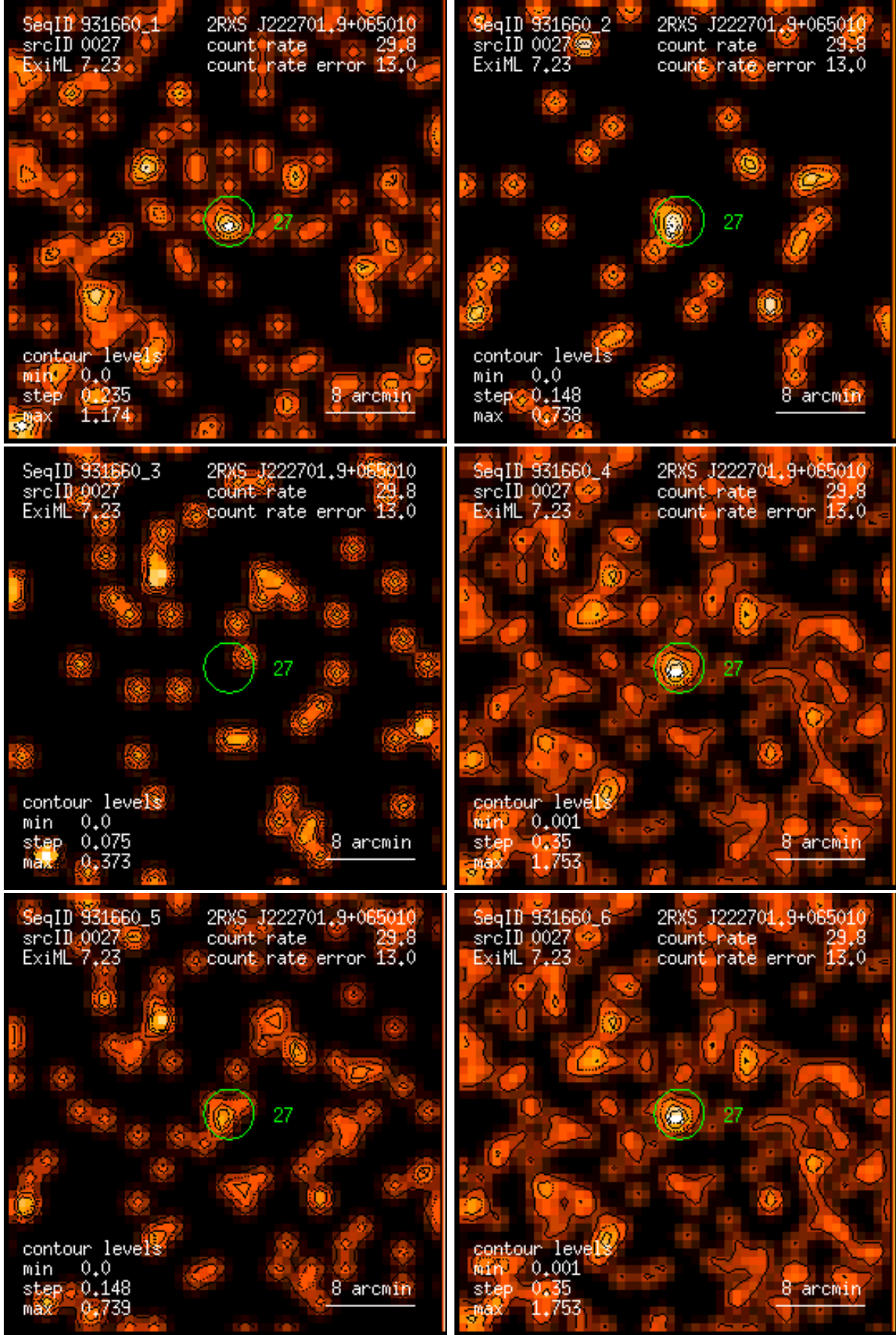
Figure 27: RASS 931660: detection 0027: band rate images, Gaussian filter: (1) PSPC channels 11 – 41, (2) 52 – 90, (3) 91 – 201, (4) 11 – 235, (5) 52 – 201, (6) 11 – 201. Broad band rates in counts/ks. Band rate contour levels in counts/ks/arcmin 2 .
