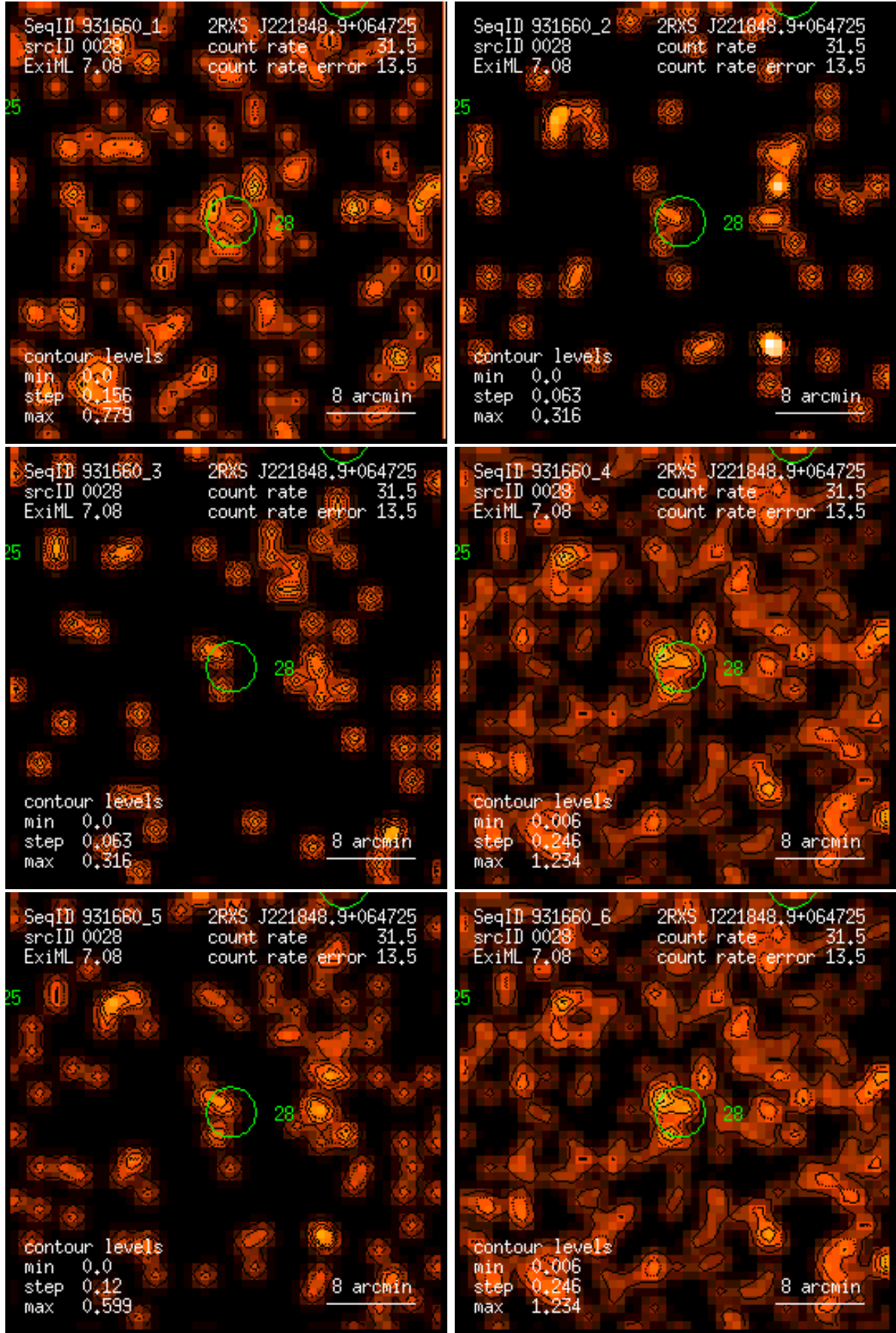
Figure 28: RASS 931660: detection 0028: band rate images, Gaussian filter: (1) PSPC channels 11 – 41, (2) 52 – 90, (3) 91 – 201, (4) 11 – 235, (5) 52 – 201, (6) 11 – 201. Broad band rates in counts/ks. Band rate contour levels in counts/ks/arcmin 2 .
