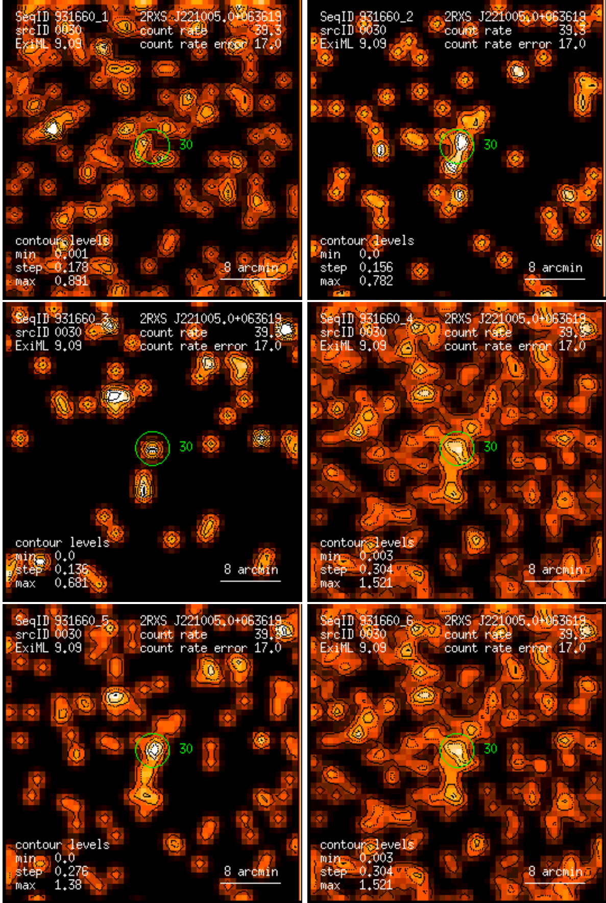
Figure 30: RASS 931660: detection 0030: band rate images, Gaussian filter: (1) PSPC channels 11 – 41, (2) 52 – 90, (3) 91 – 201, (4) 11 – 235, (5) 52 – 201, (6) 11 – 201. Broad band rates in counts/ks. Band rate contour levels in counts/ks/arcmin 2 .
