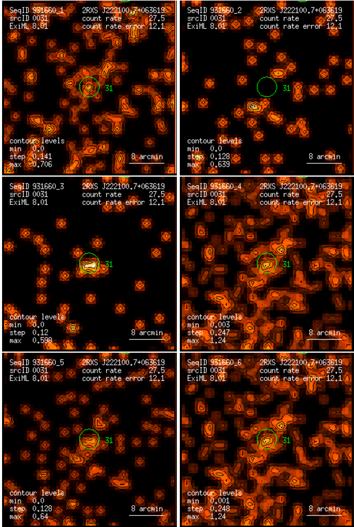
Figure 31: RASS 931660: detection 0031: band rate images, Gaussian filter: (1) PSPC channels 11 – 41, (2) 52 – 90, (3) 91 – 201, (4) 11 – 235, (5) 52 – 201, (6) 11 – 201. Broad band rates in counts/ks. Band rate contour levels in counts/ks/arcmin 2 .
