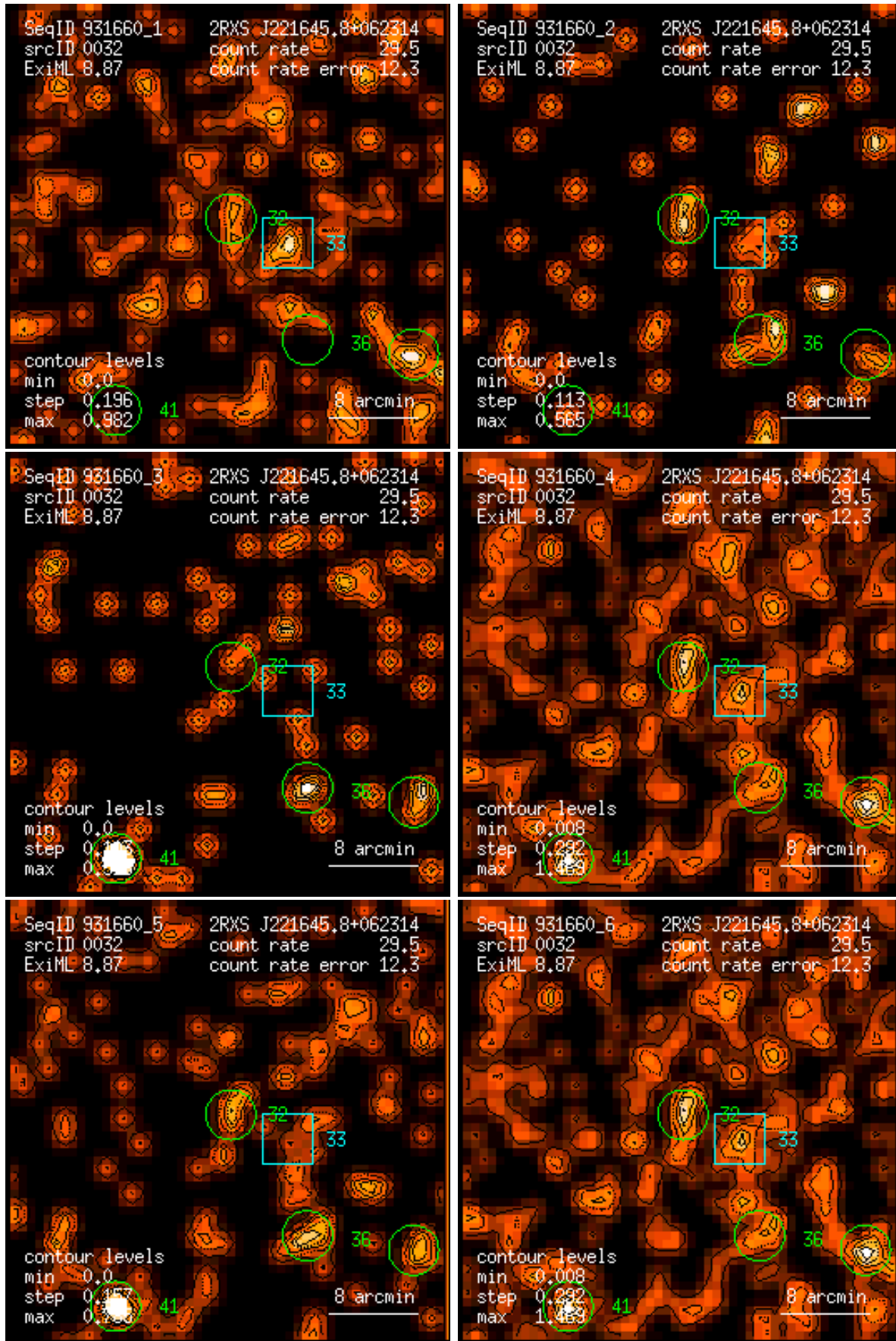
Figure 32: RASS 931660: detection 0032: band rate images, Gaussian filter: (1) PSPC channels 11 – 41, (2) 52 – 90, (3) 91 – 201, (4) 11 – 235, (5) 52 – 201, (6) 11 – 201. Broad band rates in counts/ks. Band rate contour levels in counts/ks/arcmin 2 .
