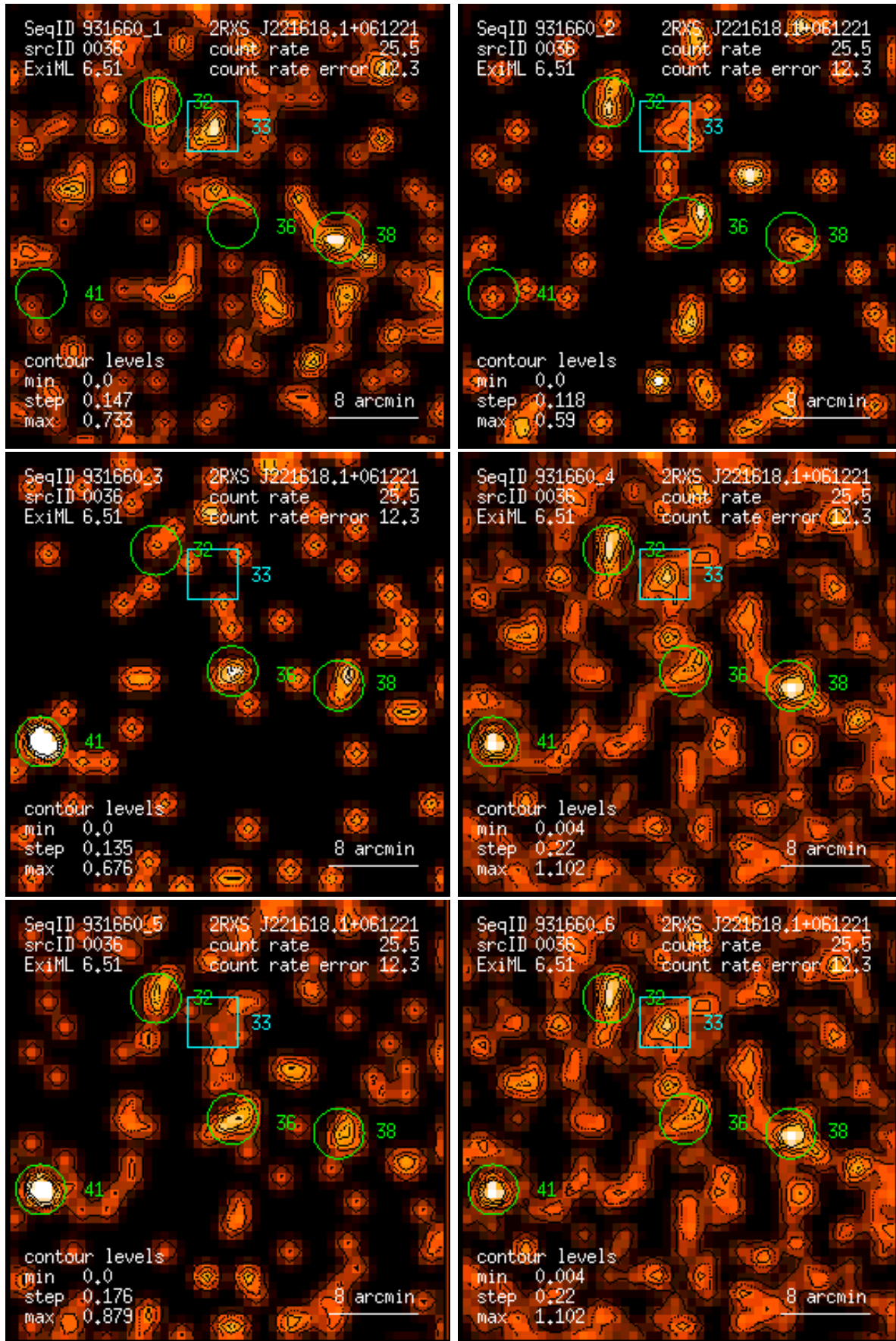
Figure 36: RASS 931660: detection 0036: band rate images, Gaussian filter: (1) PSPC channels 11 – 41, (2) 52 – 90, (3) 91 – 201, (4) 11 – 235, (5) 52 – 201, (6) 11 – 201. Broad band rates in counts/ks. Band rate contour levels in counts/ks/arcmin 2 .
