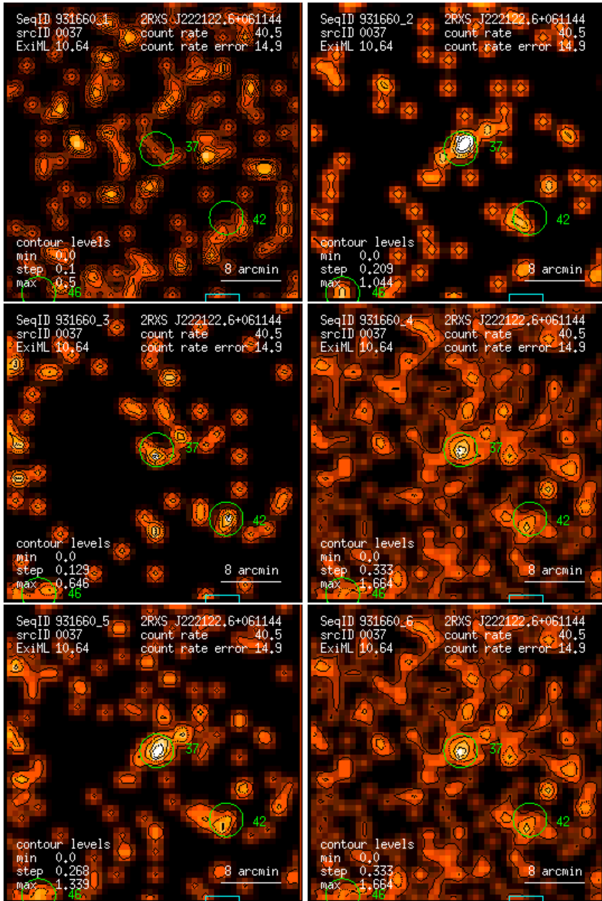
Figure 37: RASS 931660: detection 0037: band rate images, Gaussian filter: (1) PSPC channels 11 – 41, (2) 52 – 90, (3) 91 – 201, (4) 11 – 235, (5) 52 – 201, (6) 11 – 201. Broad band rates in counts/ks. Band rate contour levels in counts/ks/arcmin 2 .
