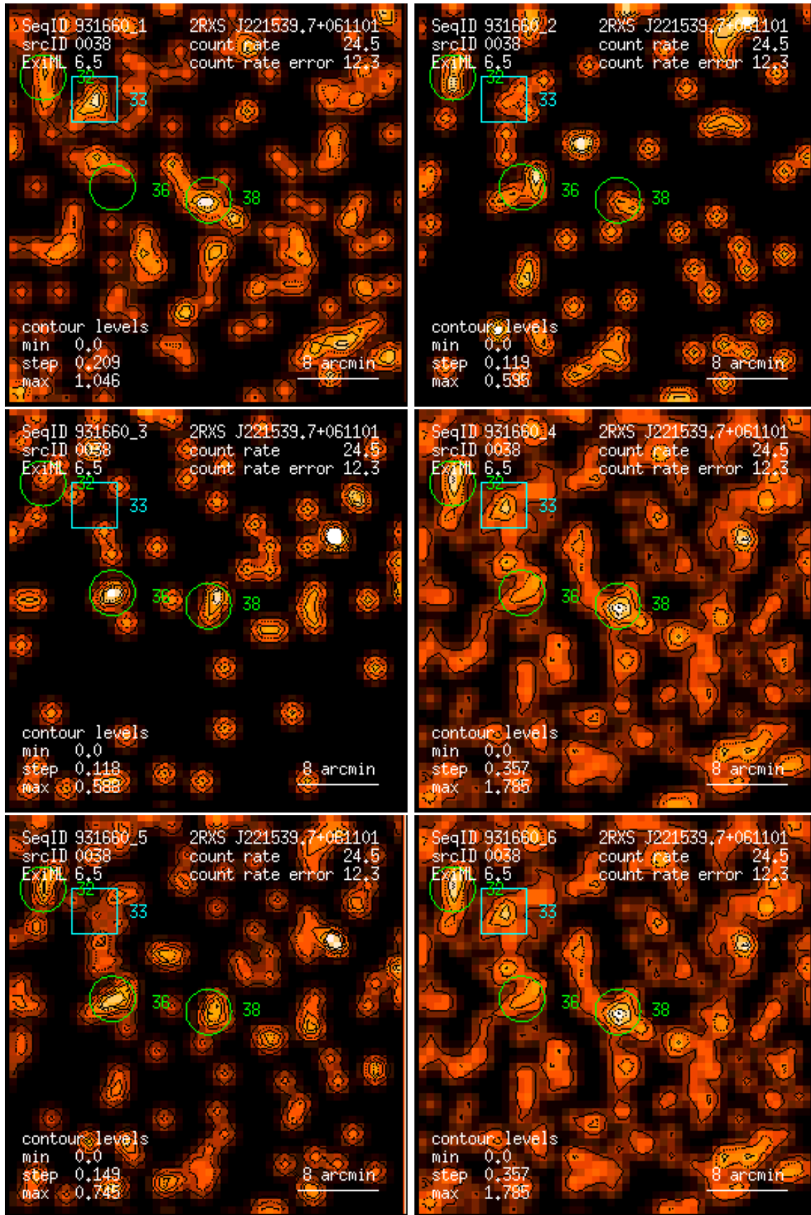
Figure 38: RASS 931660: detection 0038: band rate images, Gaussian filter: (1) PSPC channels 11 – 41, (2) 52 – 90, (3) 91 – 201, (4) 11 – 235, (5) 52 – 201, (6) 11 – 201. Broad band rates in counts/ks. Band rate contour levels in counts/ks/arcmin 2 .
