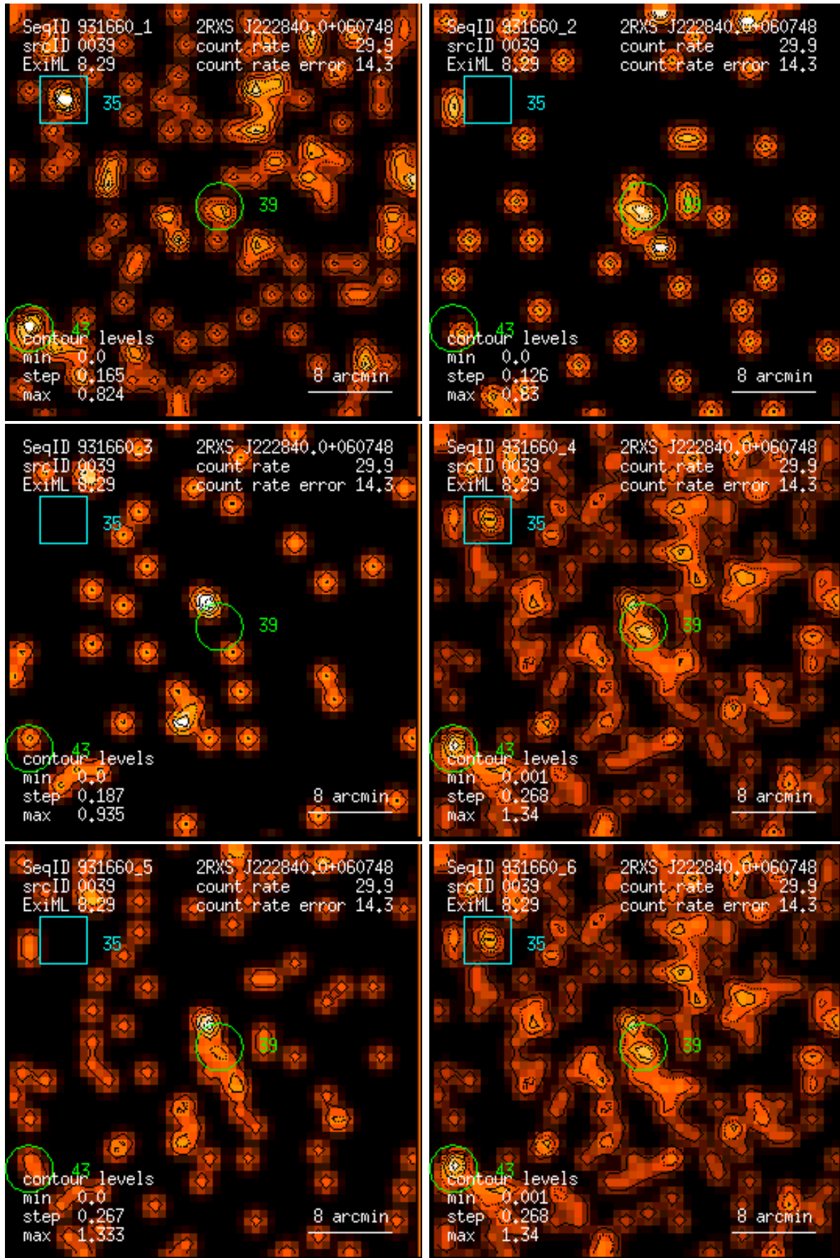
Figure 39: RASS 931660: detection 0039: band rate images, Gaussian filter: (1) PSPC channels 11 – 41, (2) 52 – 90, (3) 91 – 201, (4) 11 – 235, (5) 52 – 201, (6) 11 – 201. Broad band rates in counts/ks. Band rate contour levels in counts/ks/arcmin 2 .
