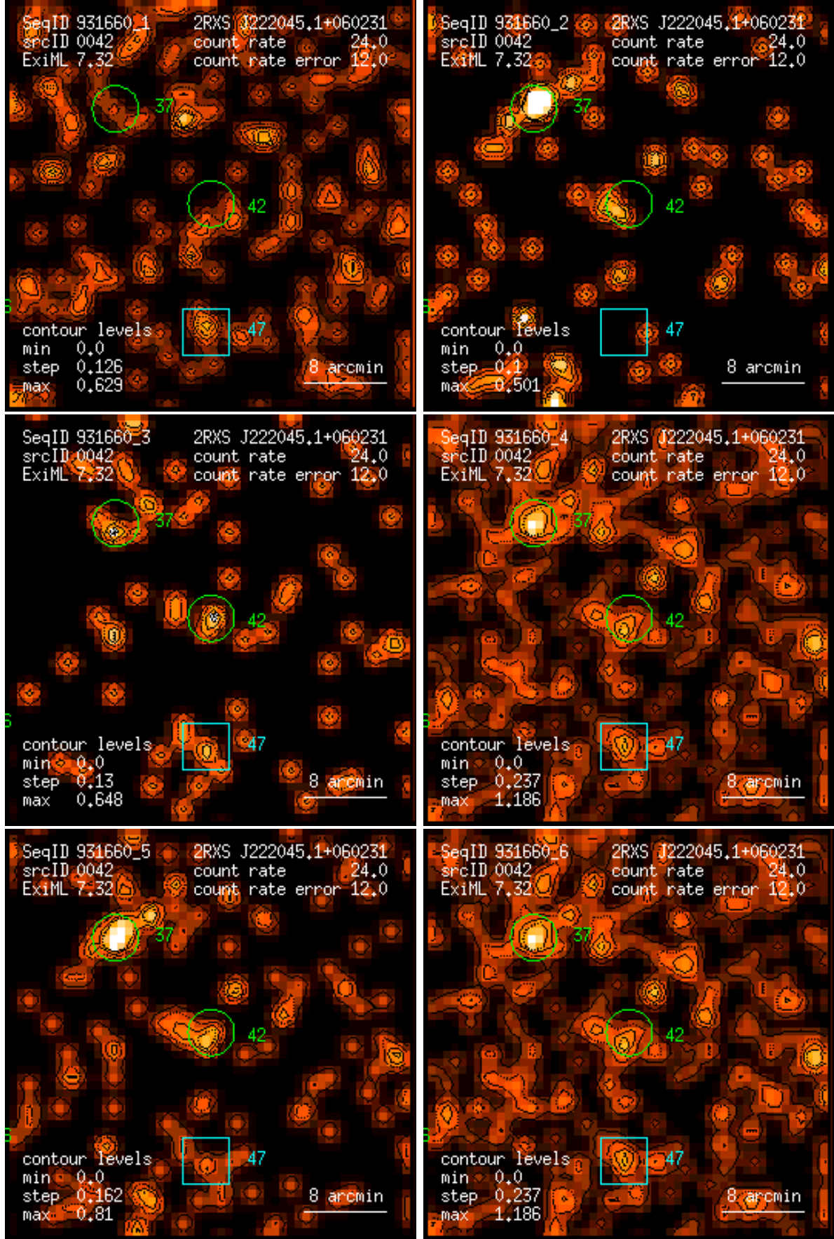
Figure 42: RASS 931660: detection 0042: band rate images, Gaussian filter: (1) PSPC channels 11 – 41, (2) 52 – 90, (3) 91 – 201, (4) 11 – 235, (5) 52 – 201, (6) 11 – 201. Broad band rates in counts/ks. Band rate contour levels in counts/ks/arcmin 2 .
