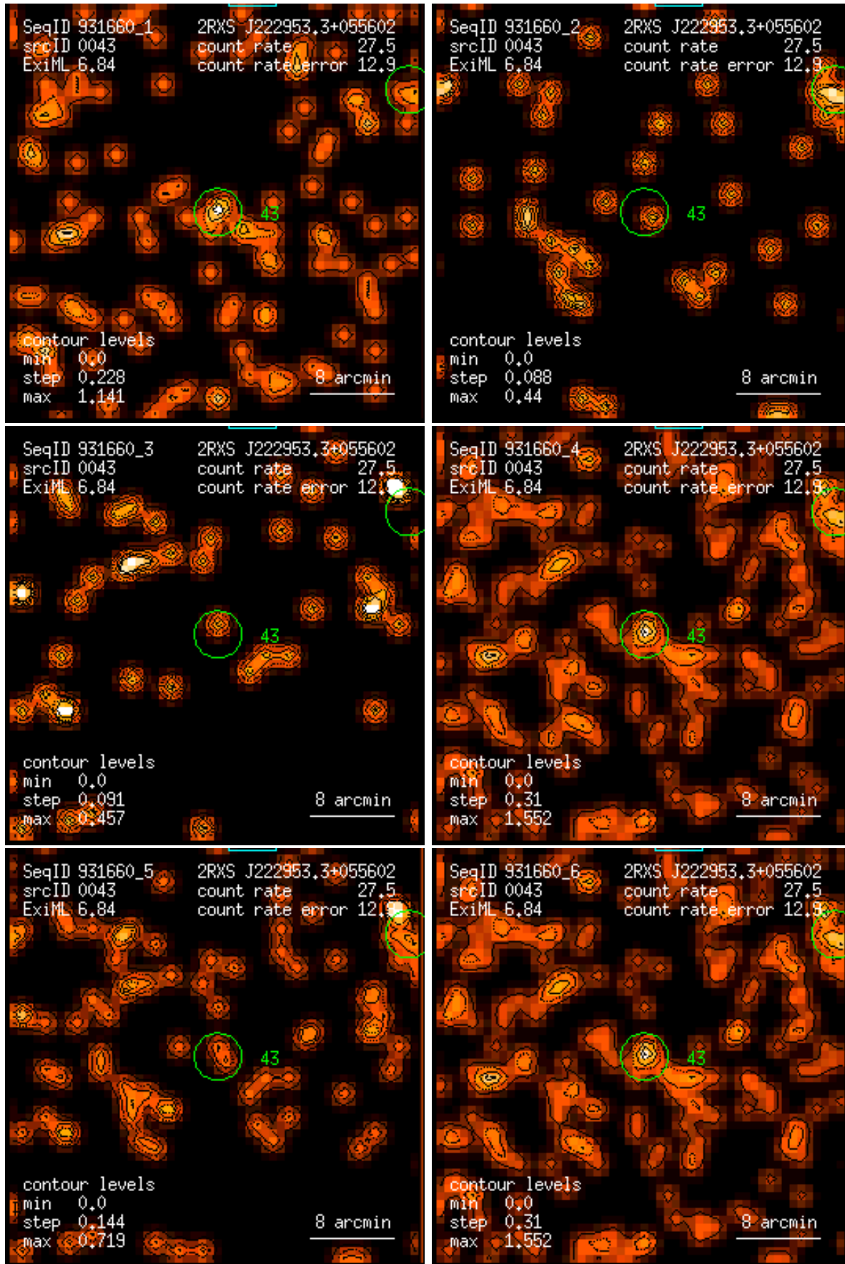
Figure 43: RASS 931660: detection 0043: band rate images, Gaussian filter: (1) PSPC channels 11 – 41, (2) 52 – 90, (3) 91 – 201, (4) 11 – 235, (5) 52 – 201, (6) 11 – 201. Broad band rates in counts/ks. Band rate contour levels in counts/ks/arcmin 2 .
