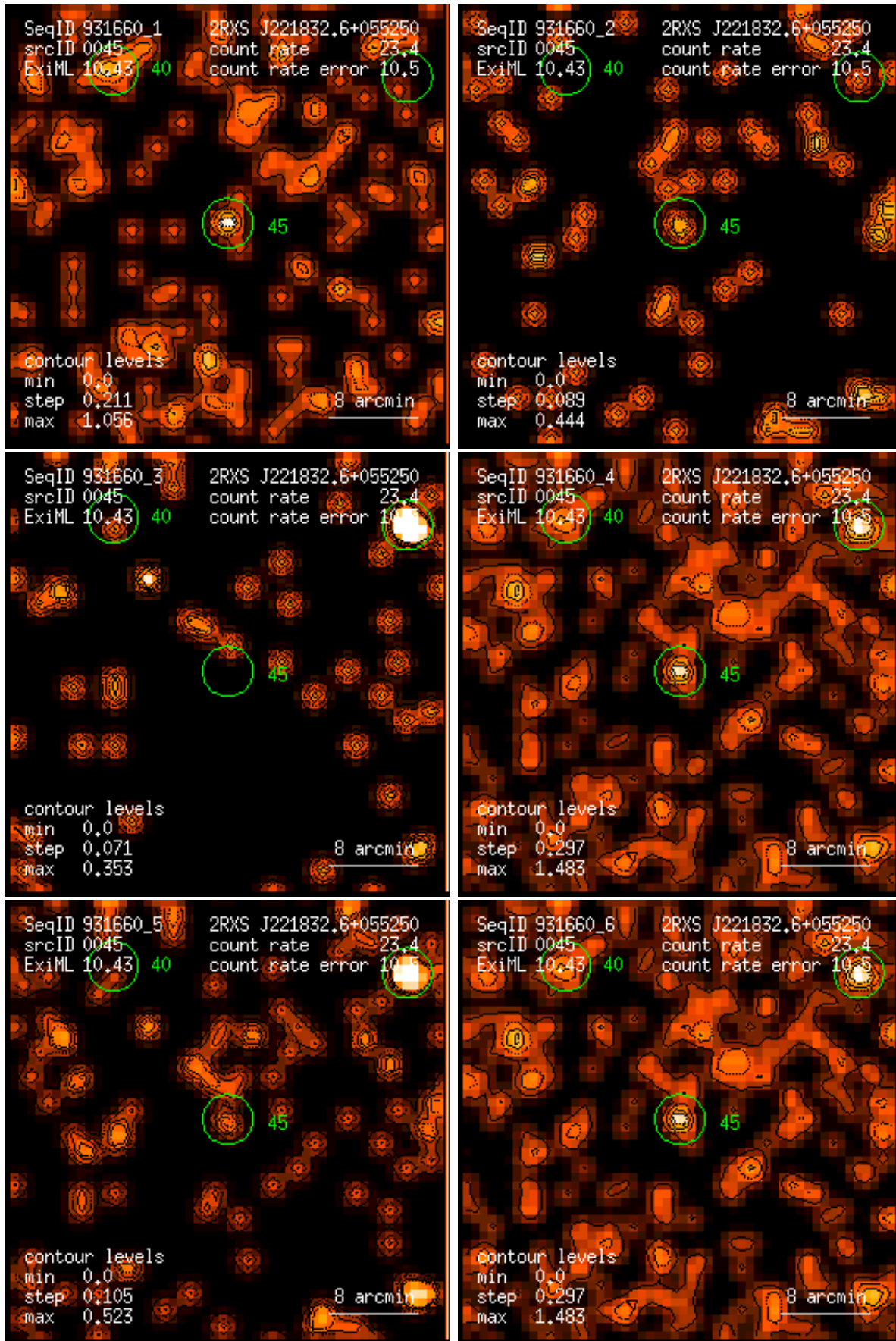
Figure 45: RASS 931660: detection 0045: band rate images, Gaussian filter: (1) PSPC channels 11 – 41, (2) 52 – 90, (3) 91 – 201, (4) 11 – 235, (5) 52 – 201, (6) 11 – 201. Broad band rates in counts/ks. Band rate contour levels in counts/ks/arcmin 2 .
