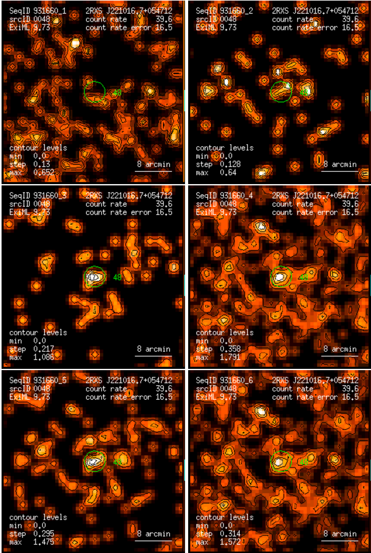
Figure 48: RASS 931660: detection 0048: band rate images, Gaussian filter: (1) PSPC channels 11 – 41, (2) 52 – 90, (3) 91 – 201, (4) 11 – 235, (5) 52 – 201, (6) 11 – 201. Broad band rates in counts/ks. Band rate contour levels in counts/ks/arcmin 2 .
