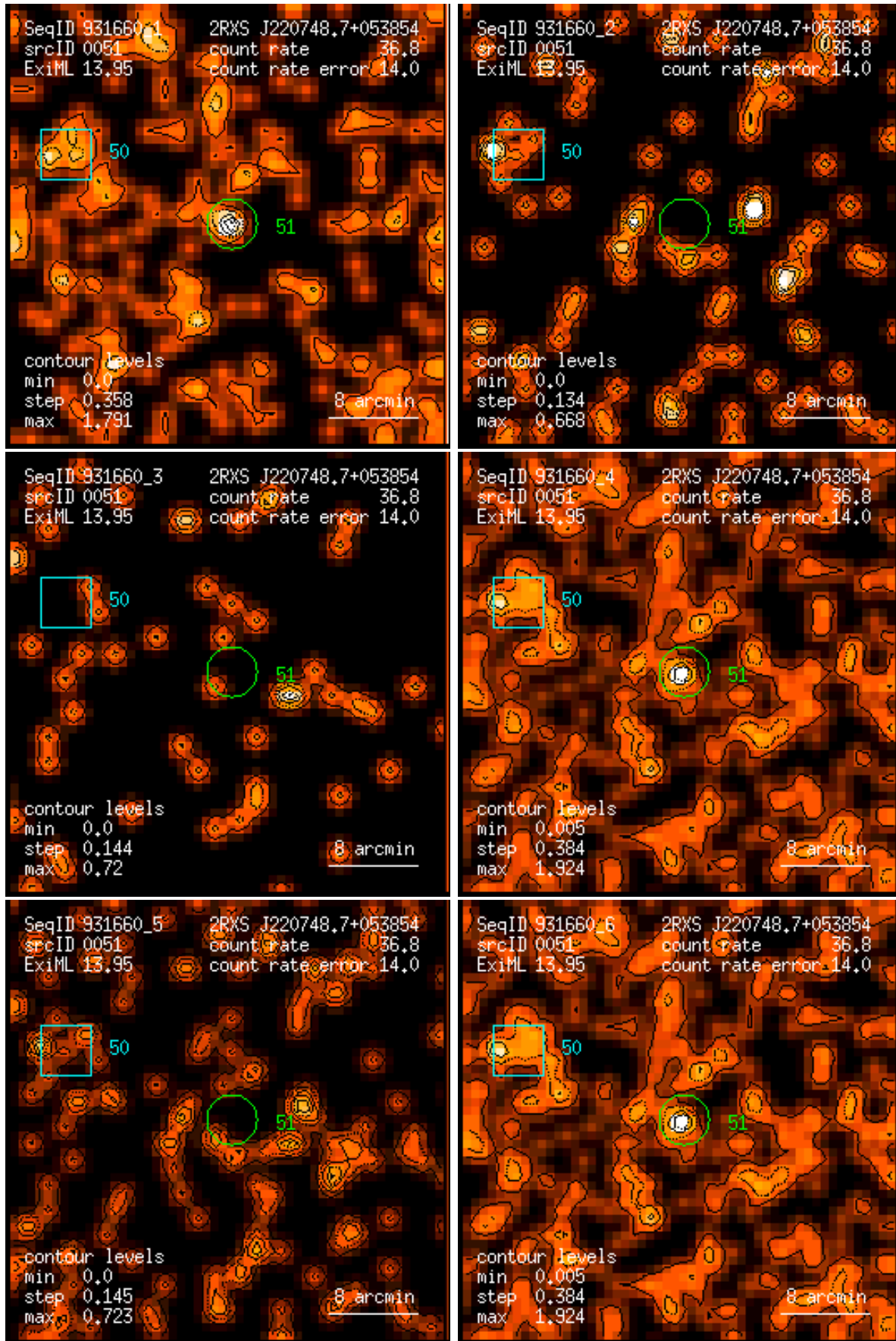
Figure 51: RASS 931660: detection 0051: band rate images, Gaussian filter: (1) PSPC channels 11 – 41, (2) 52 – 90, (3) 91 – 201, (4) 11 – 235, (5) 52 – 201, (6) 11 – 201. Broad band rates in counts/ks. Band rate contour levels in counts/ks/arcmin 2 .
