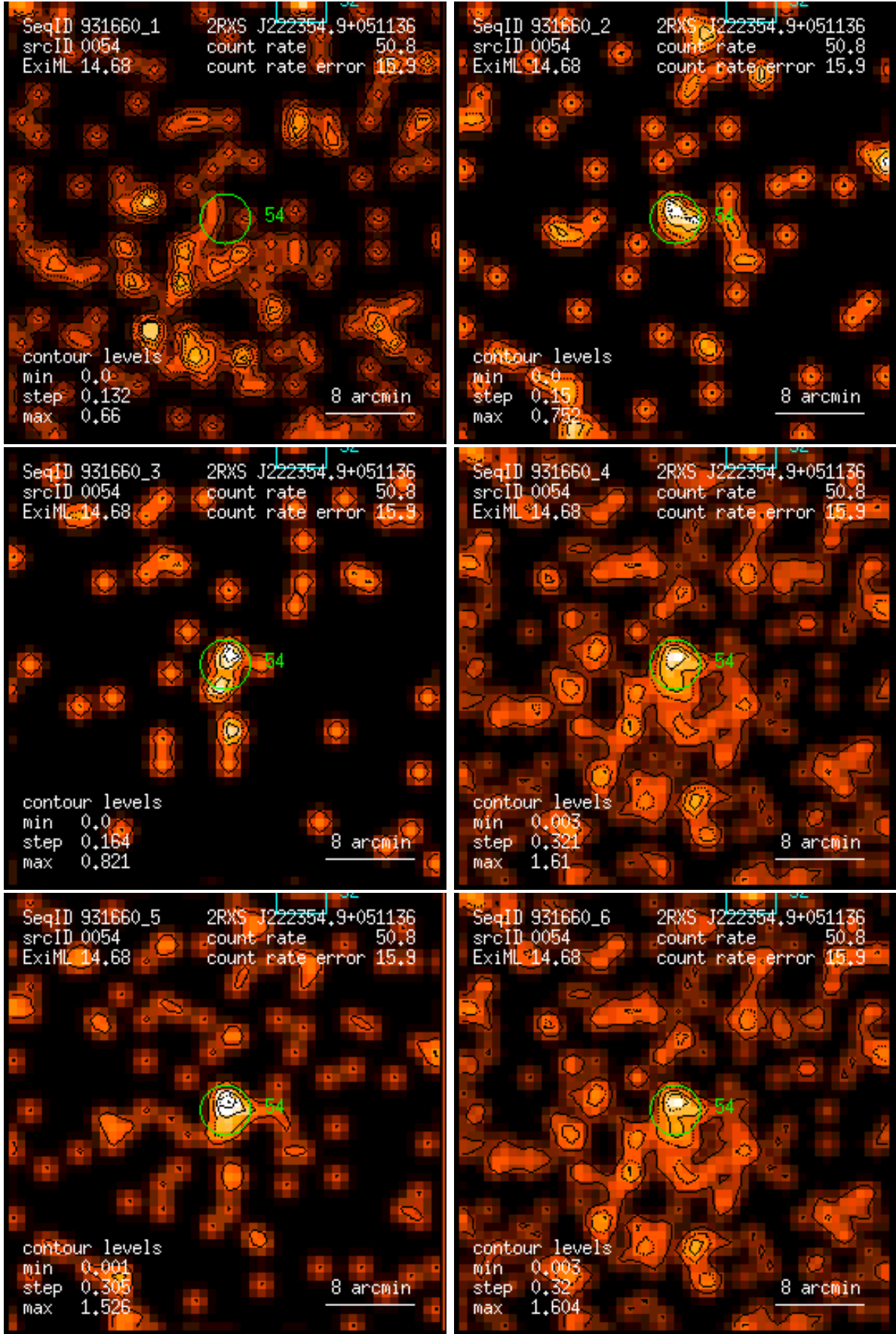
Figure 54: RASS 931660: detection 0054: band rate images, Gaussian filter: (1) PSPC channels 11 – 41, (2) 52 – 90, (3) 91 – 201, (4) 11 – 235, (5) 52 – 201, (6) 11 – 201. Broad band rates in counts/ks. Band rate contour levels in counts/ks/arcmin 2 .
