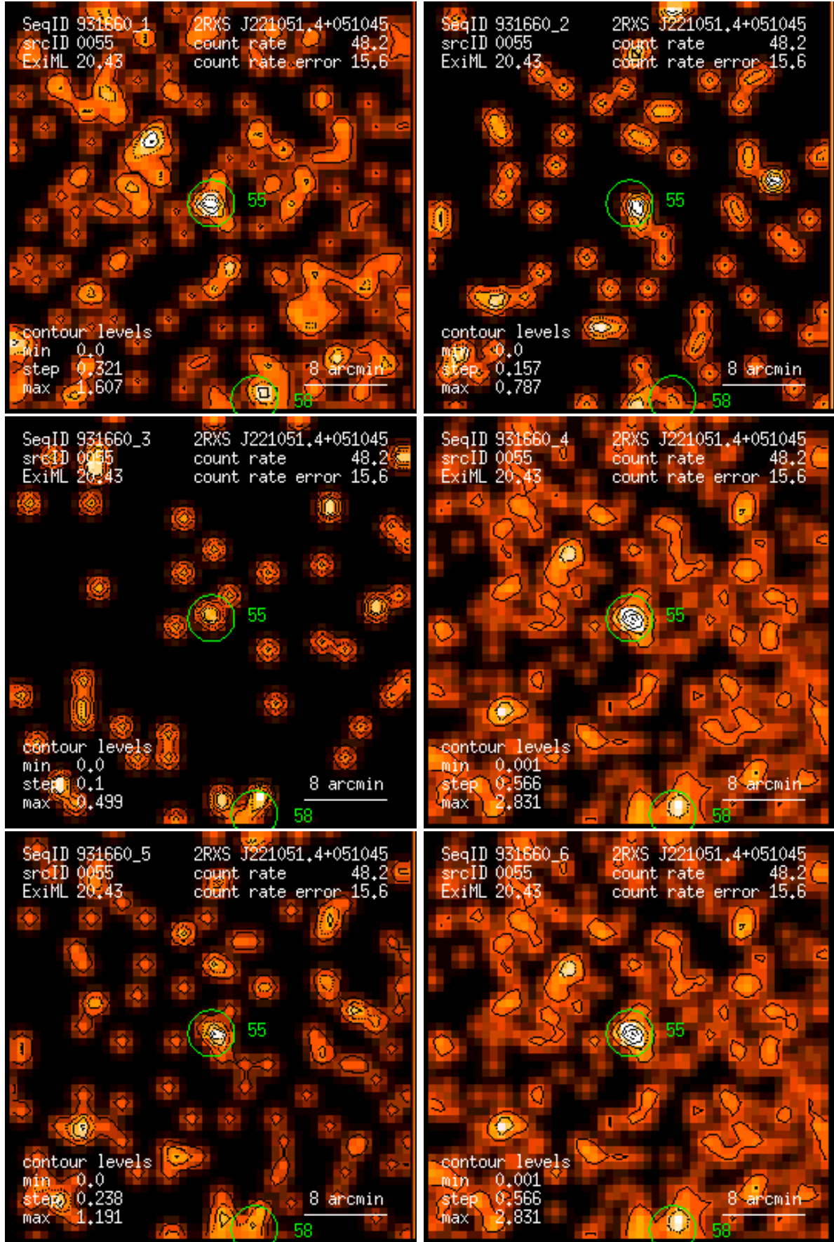
Figure 55: RASS 931660: detection 0055: band rate images, Gaussian filter: (1) PSPC channels 11 – 41, (2) 52 – 90, (3) 91 – 201, (4) 11 – 235, (5) 52 – 201, (6) 11 – 201. Broad band rates in counts/ks. Band rate contour levels in counts/ks/arcmin 2 .
