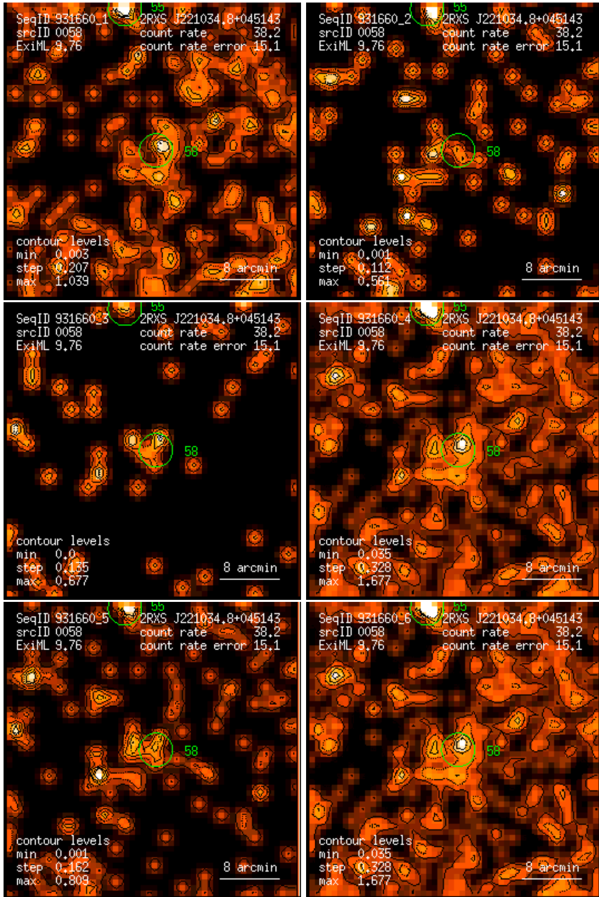
Figure 58: RASS 931660: detection 0058: band rate images, Gaussian filter: (1) PSPC channels 11 – 41, (2) 52 – 90, (3) 91 – 201, (4) 11 – 235, (5) 52 – 201, (6) 11 – 201. Broad band rates in counts/ks. Band rate contour levels in counts/ks/arcmin 2 .
