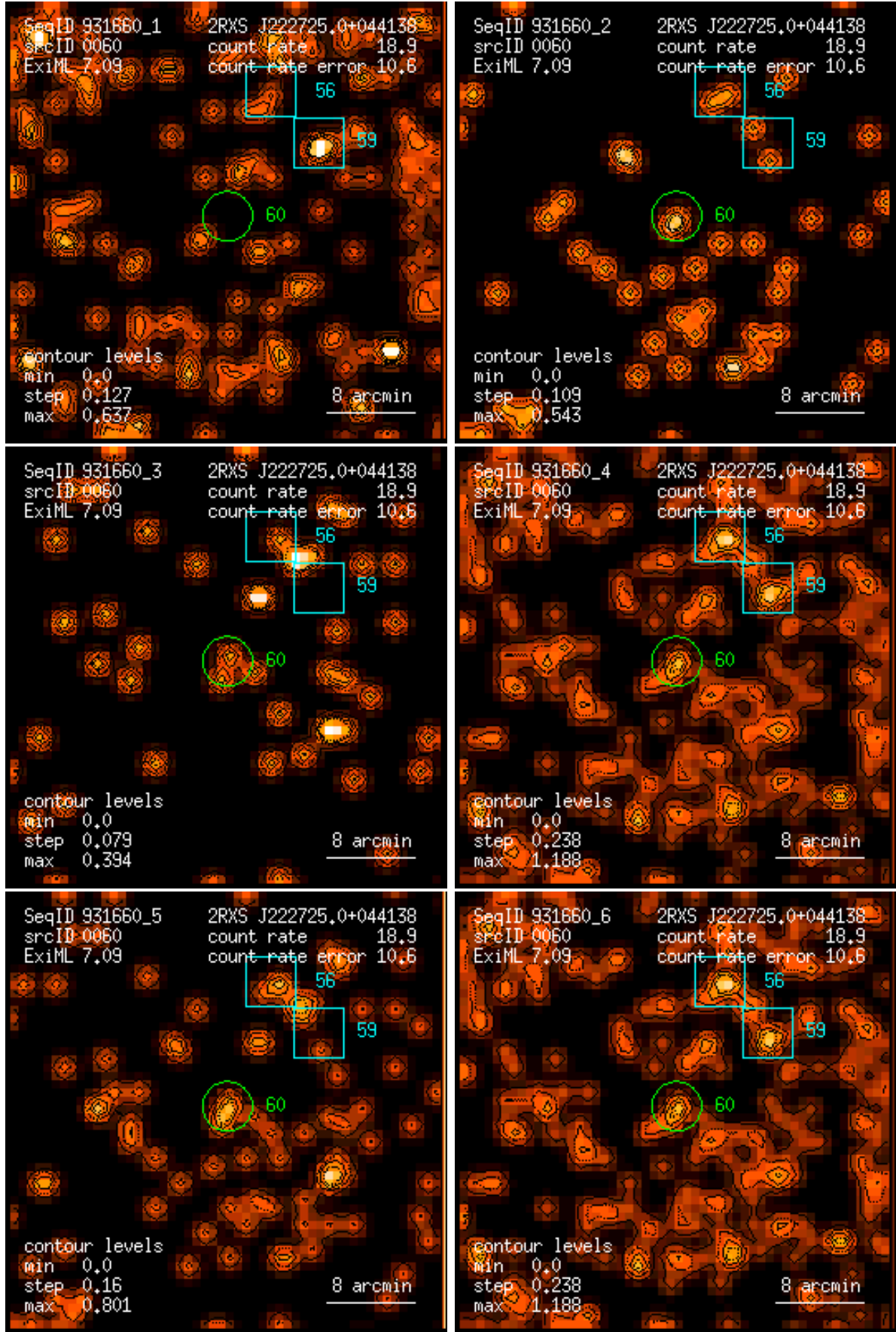
Figure 60: RASS 931660: detection 0060: band rate images, Gaussian filter: (1) PSPC channels 11 – 41, (2) 52 – 90, (3) 91 – 201, (4) 11 – 235, (5) 52 – 201, (6) 11 – 201. Broad band rates in counts/ks. Band rate contour levels in counts/ks/arcmin 2 .
