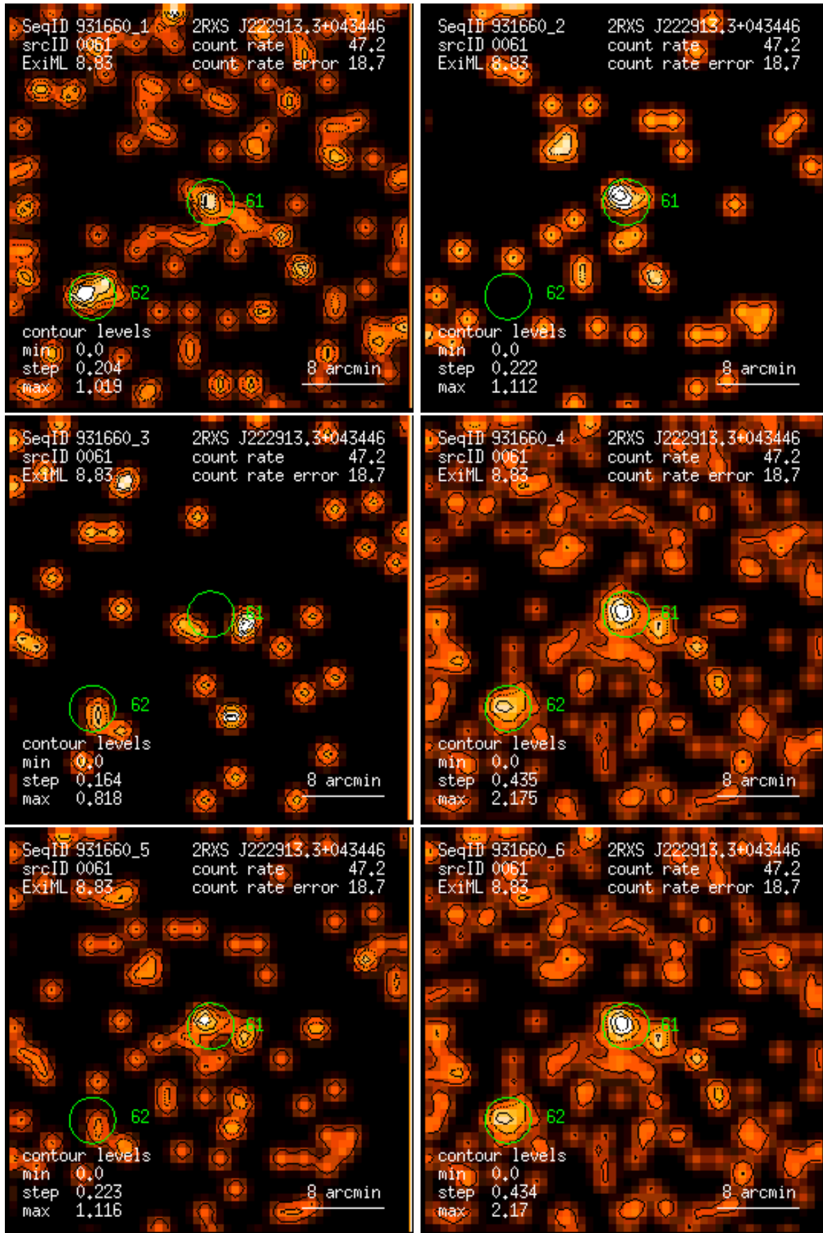
Figure 61: RASS 931660: detection 0061: band rate images, Gaussian filter: (1) PSPC channels 11 – 41, (2) 52 – 90, (3) 91 – 201, (4) 11 – 235, (5) 52 – 201, (6) 11 – 201. Broad band rates in counts/ks. Band rate contour levels in counts/ks/arcmin 2 .
