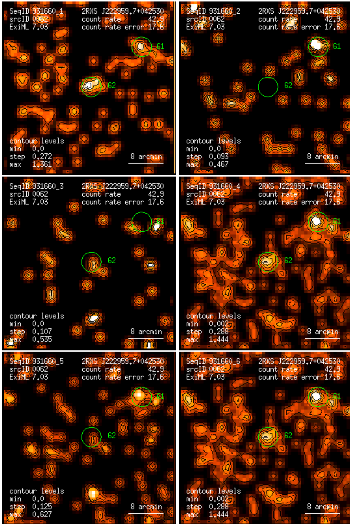
Figure 62: RASS 931660: detection 0062: band rate images, Gaussian filter: (1) PSPC channels 11 – 41, (2) 52 – 90, (3) 91 – 201, (4) 11 – 235, (5) 52 – 201, (6) 11 – 201. Broad band rates in counts/ks. Band rate contour levels in counts/ks/arcmin 2 .
