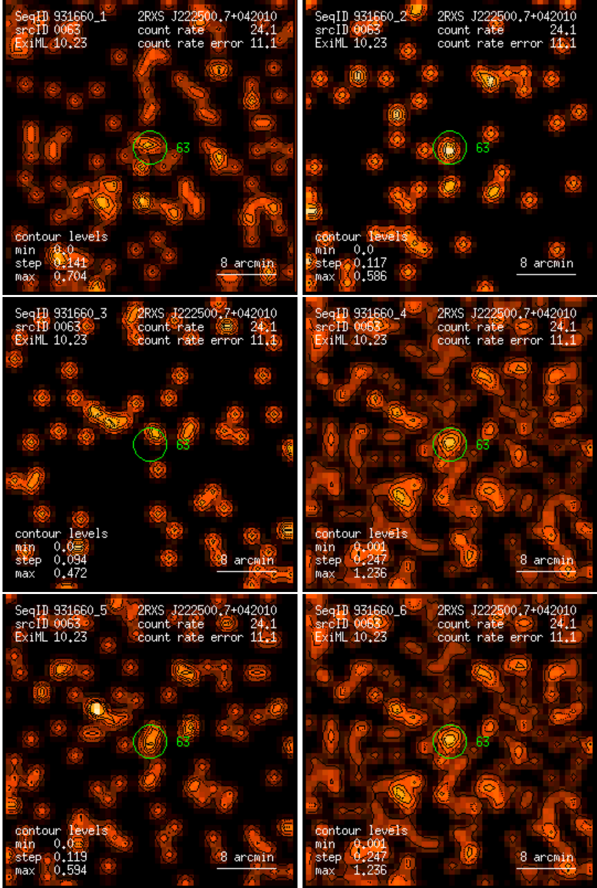
Figure 63: RASS 931660: detection 0063: band rate images, Gaussian filter: (1) PSPC channels 11 – 41, (2) 52 – 90, (3) 91 – 201, (4) 11 – 235, (5) 52 – 201, (6) 11 – 201. Broad band rates in counts/ks. Band rate contour levels in counts/ks/arcmin 2 .
