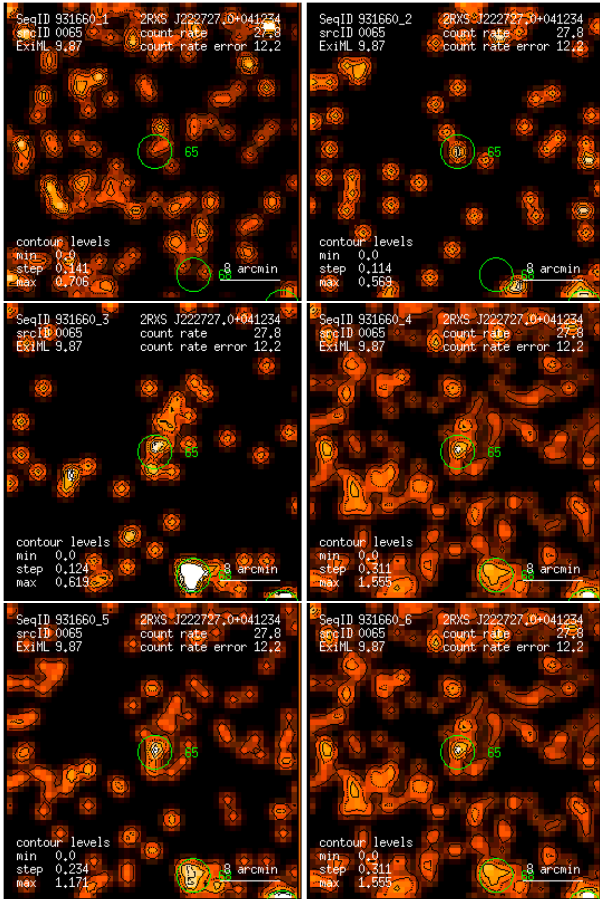
Figure 65: RASS 931660: detection 0065: band rate images, Gaussian filter: (1) PSPC channels 11 – 41, (2) 52 – 90, (3) 91 – 201, (4) 11 – 235, (5) 52 – 201, (6) 11 – 201. Broad band rates in counts/ks. Band rate contour levels in counts/ks/arcmin 2 .
