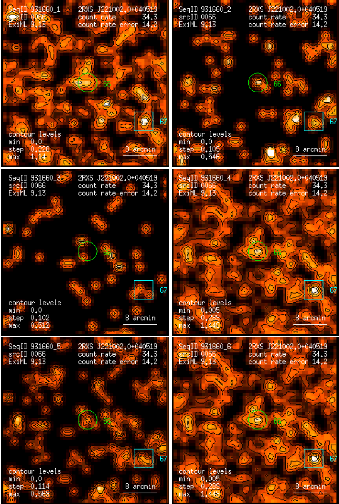
Figure 66: RASS 931660: detection 0066: band rate images, Gaussian filter: (1) PSPC channels 11 – 41, (2) 52 – 90, (3) 91 – 201, (4) 11 – 235, (5) 52 – 201, (6) 11 – 201. Broad band rates in counts/ks. Band rate contour levels in counts/ks/arcmin 2 .
