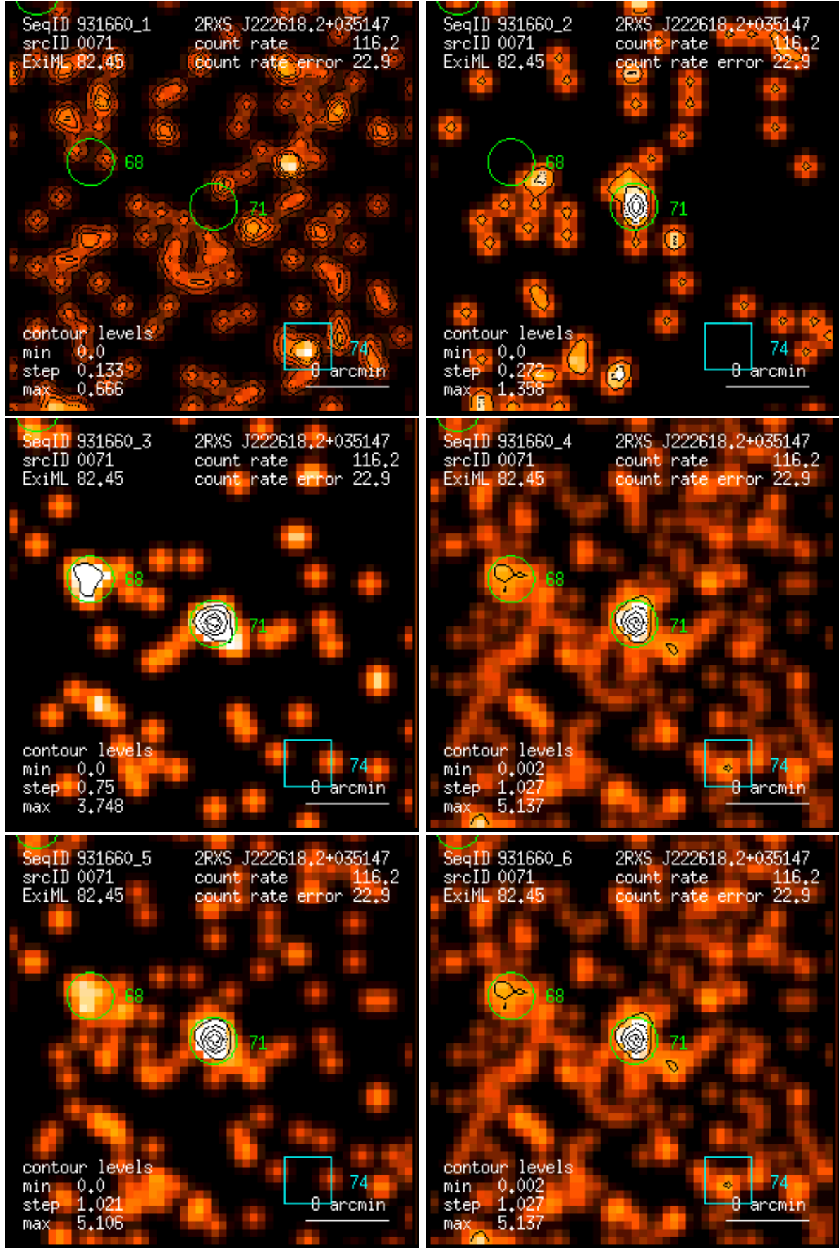
Figure 71: RASS 931660: detection 0071: band rate images, Gaussian filter: (1) PSPC channels 11 – 41, (2) 52 – 90, (3) 91 – 201, (4) 11 – 235, (5) 52 – 201, (6) 11 – 201. Broad band rates in counts/ks. Band rate contour levels in counts/ks/arcmin 2 .
