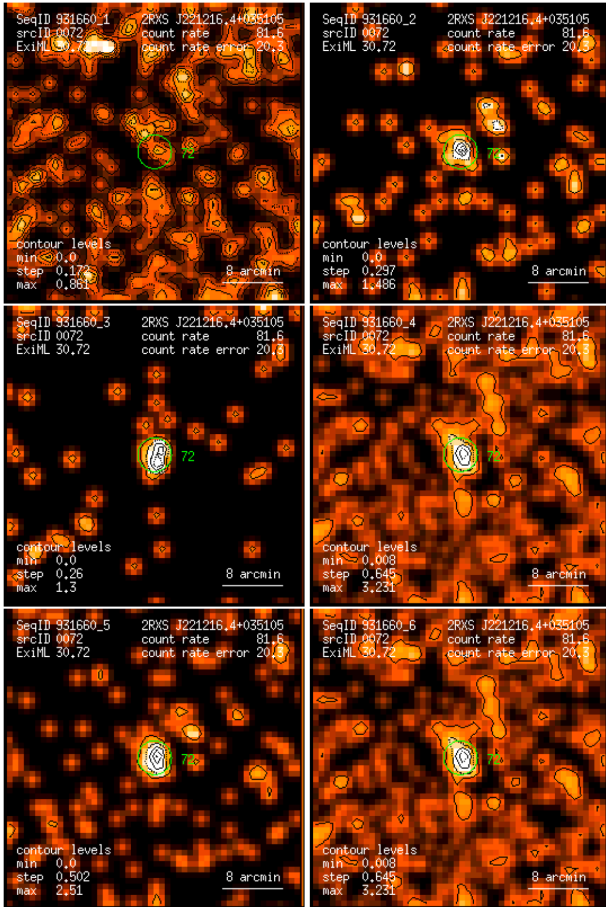
Figure 72: RASS 931660: detection 0072: band rate images, Gaussian filter: (1) PSPC channels 11 – 41, (2) 52 – 90, (3) 91 – 201, (4) 11 – 235, (5) 52 – 201, (6) 11 – 201. Broad band rates in counts/ks. Band rate contour levels in counts/ks/arcmin 2 .
