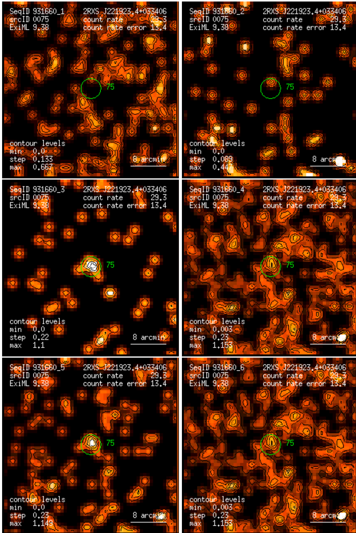
Figure 75: RASS 931660: detection 0075: band rate images, Gaussian filter: (1) PSPC channels 11 – 41, (2) 52 – 90, (3) 91 – 201, (4) 11 – 235, (5) 52 – 201, (6) 11 – 201. Broad band rates in counts/ks. Band rate contour levels in counts/ks/arcmin 2 .
